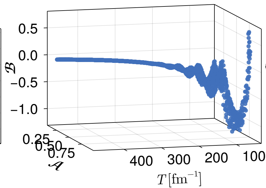
\tau = 2.5 \text{ fm}/c
