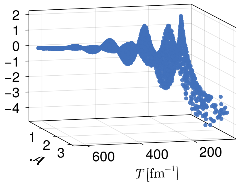
\tau = 1.0 \text{ fm}/c
