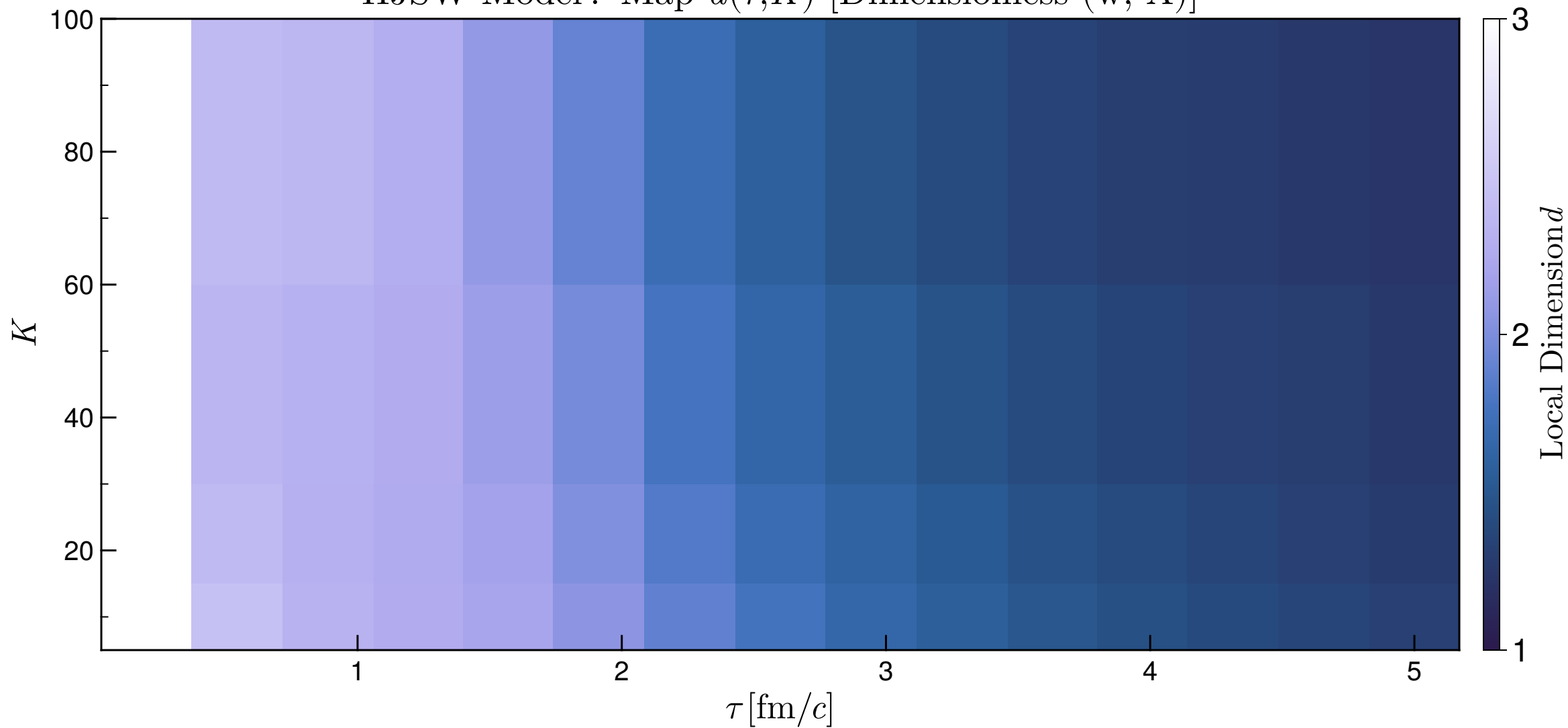
HJSW Model: Map d(\tau, K) [Dimensionless (w, A)]
