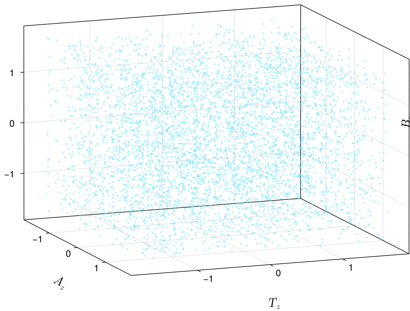
\tau = 0.45 \text{ fm}/c
