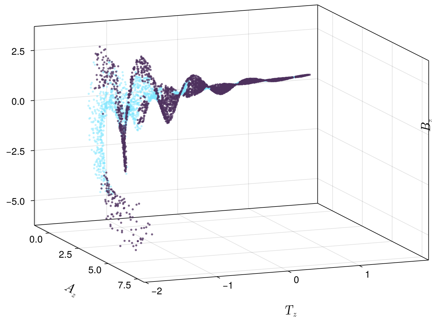
\tau = 1.0 \text{ fm}/c
