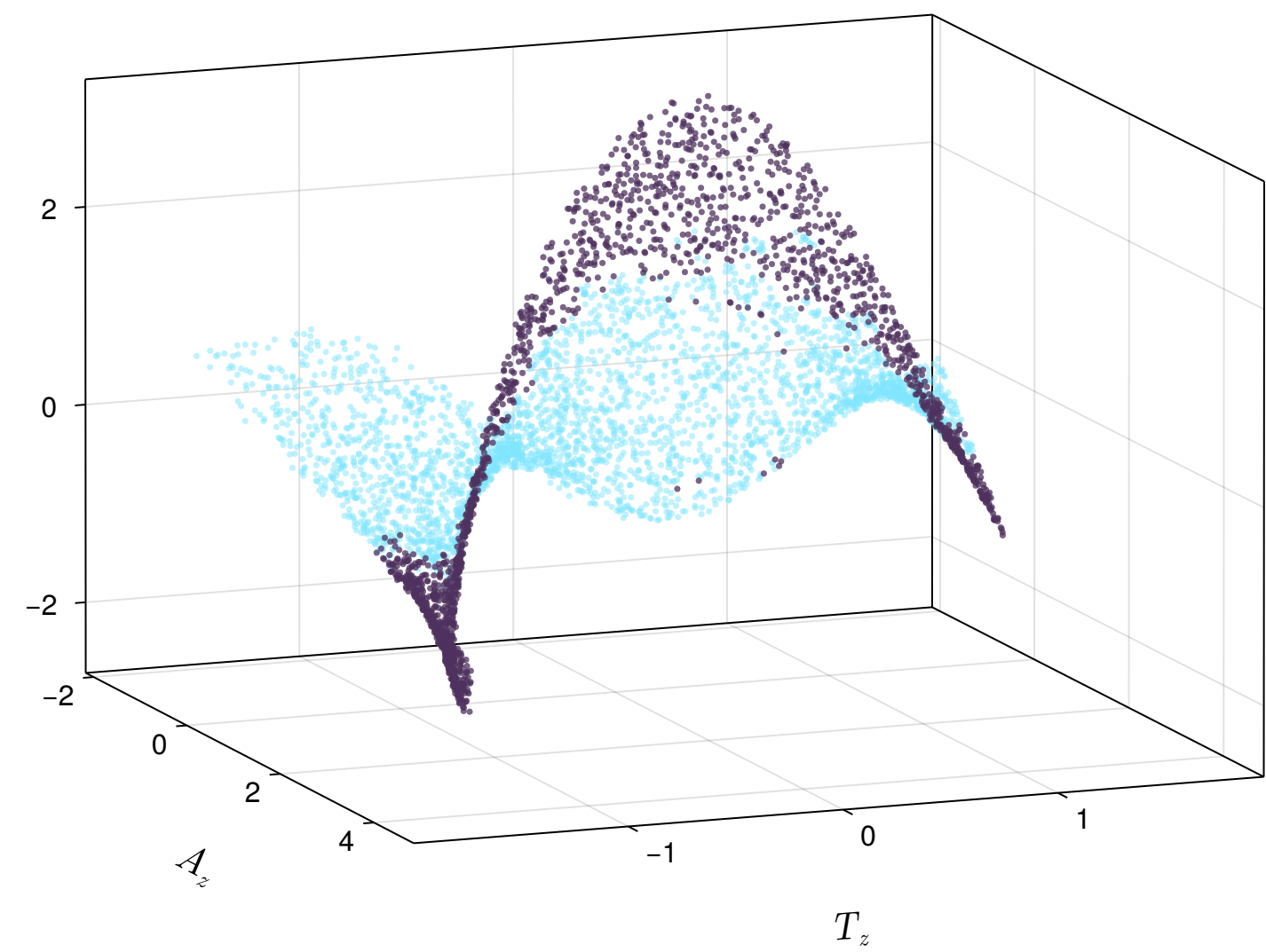
\tau = 0.65 \text{ fm}/c
