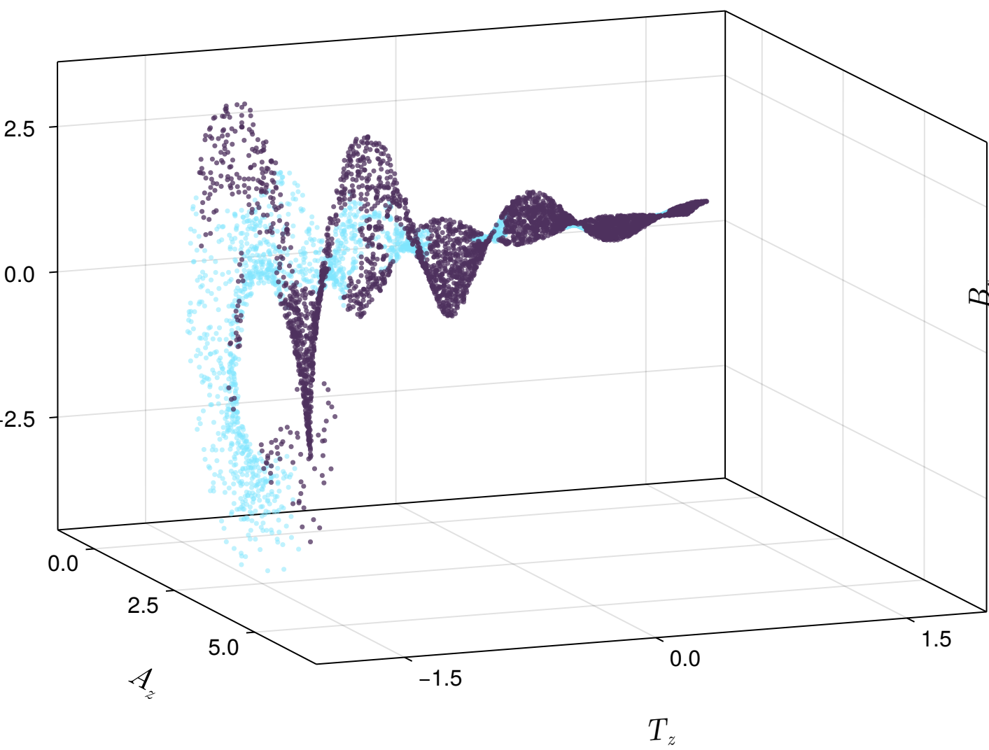
\tau = 0.8 \text{ fm}/c
