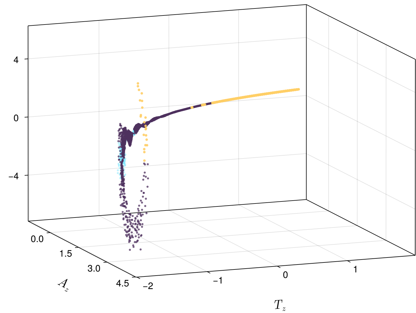
\tau = 2.5 \text{ fm}/c
