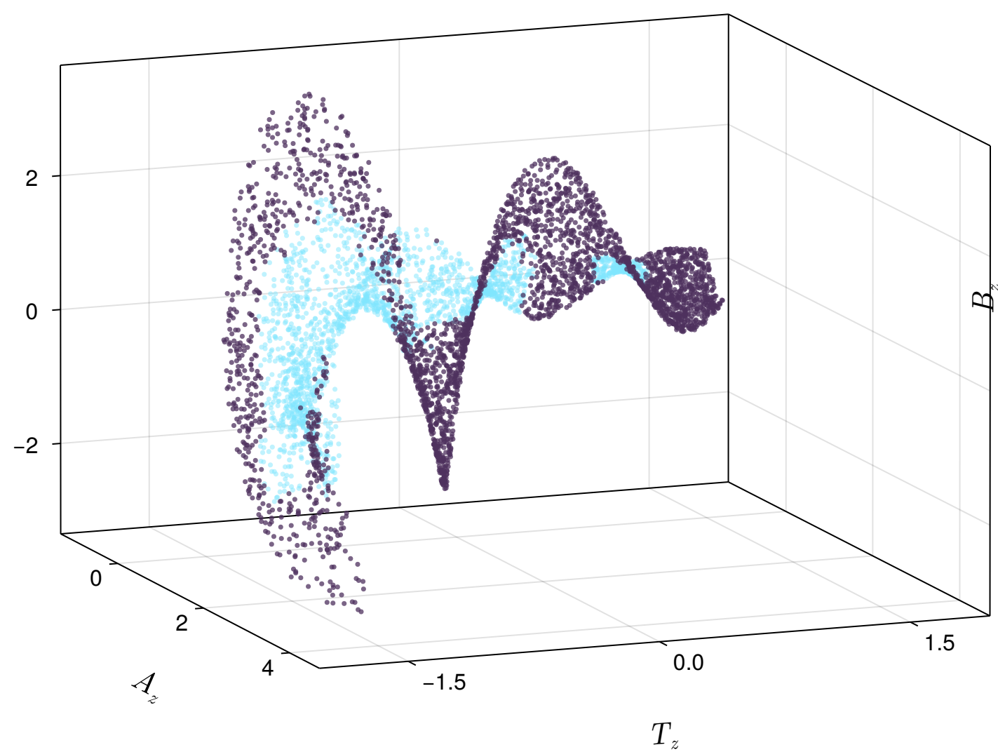
\tau = 1.0 \text{ fm}/c
