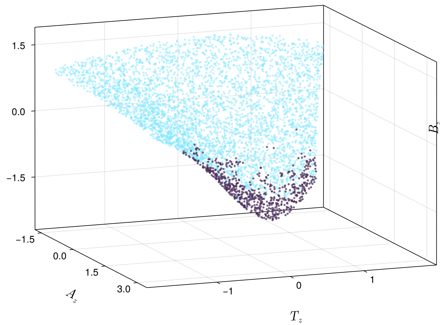
\tau = 0.55 \text{ fm}/c
