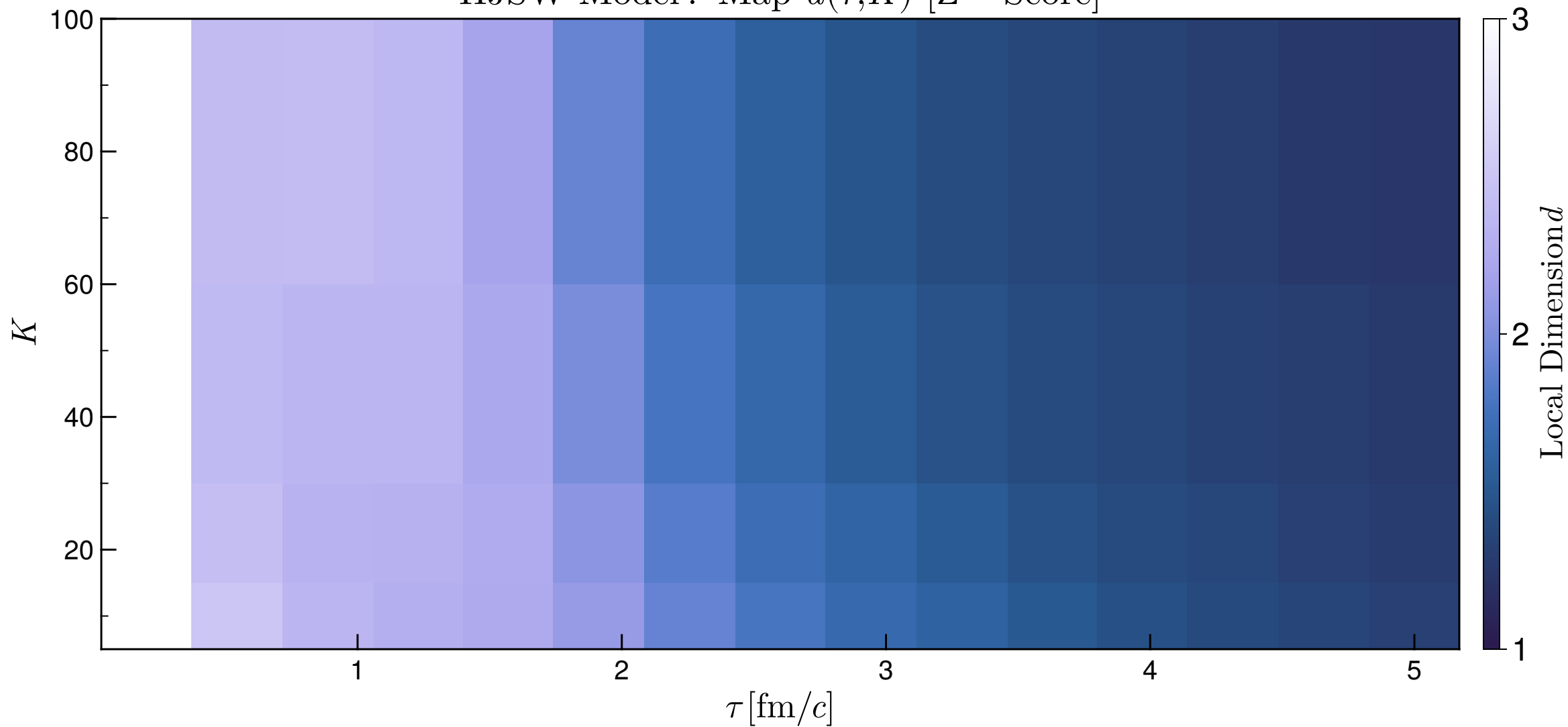
HJSW Model: Map d(\tau, K) [Z-Score]
