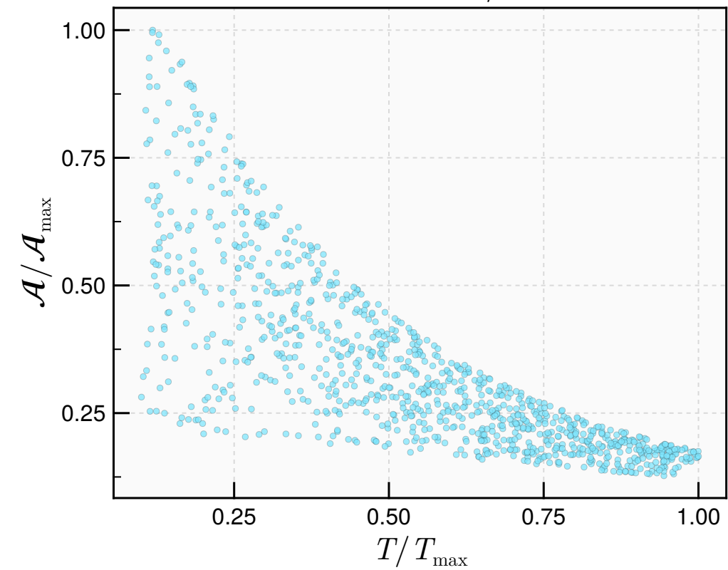
\tau = 0.65 \text{ fm}/c
