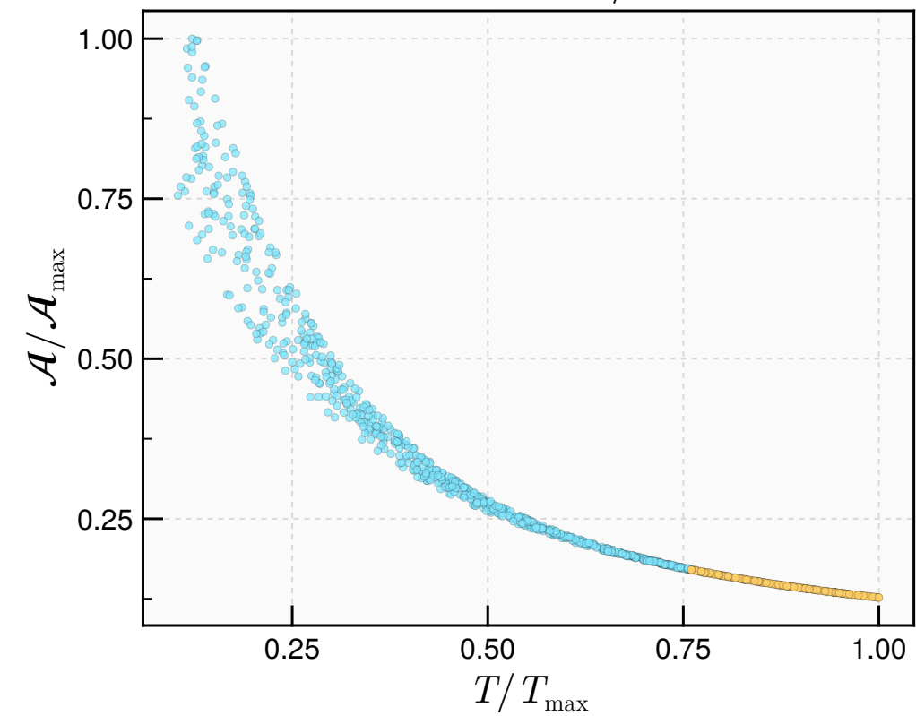
\tau = 2.5 \text{ fm}/c
