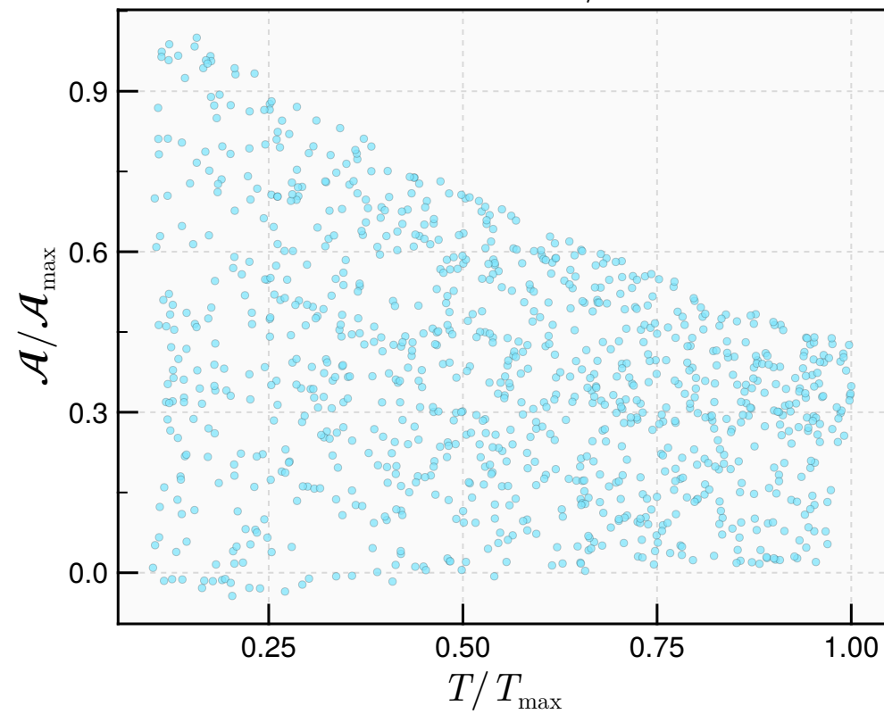
\tau = 0.55 \text{ fm}/c
