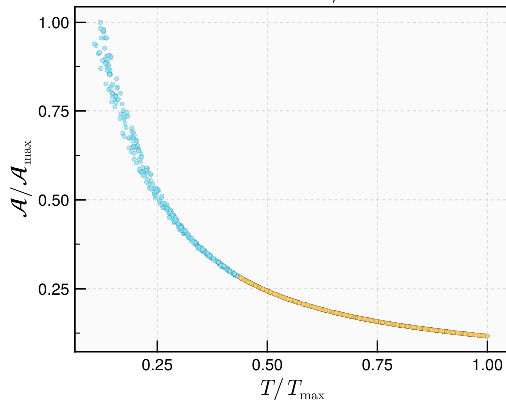
\tau = 1.0 \text{ fm}/c
