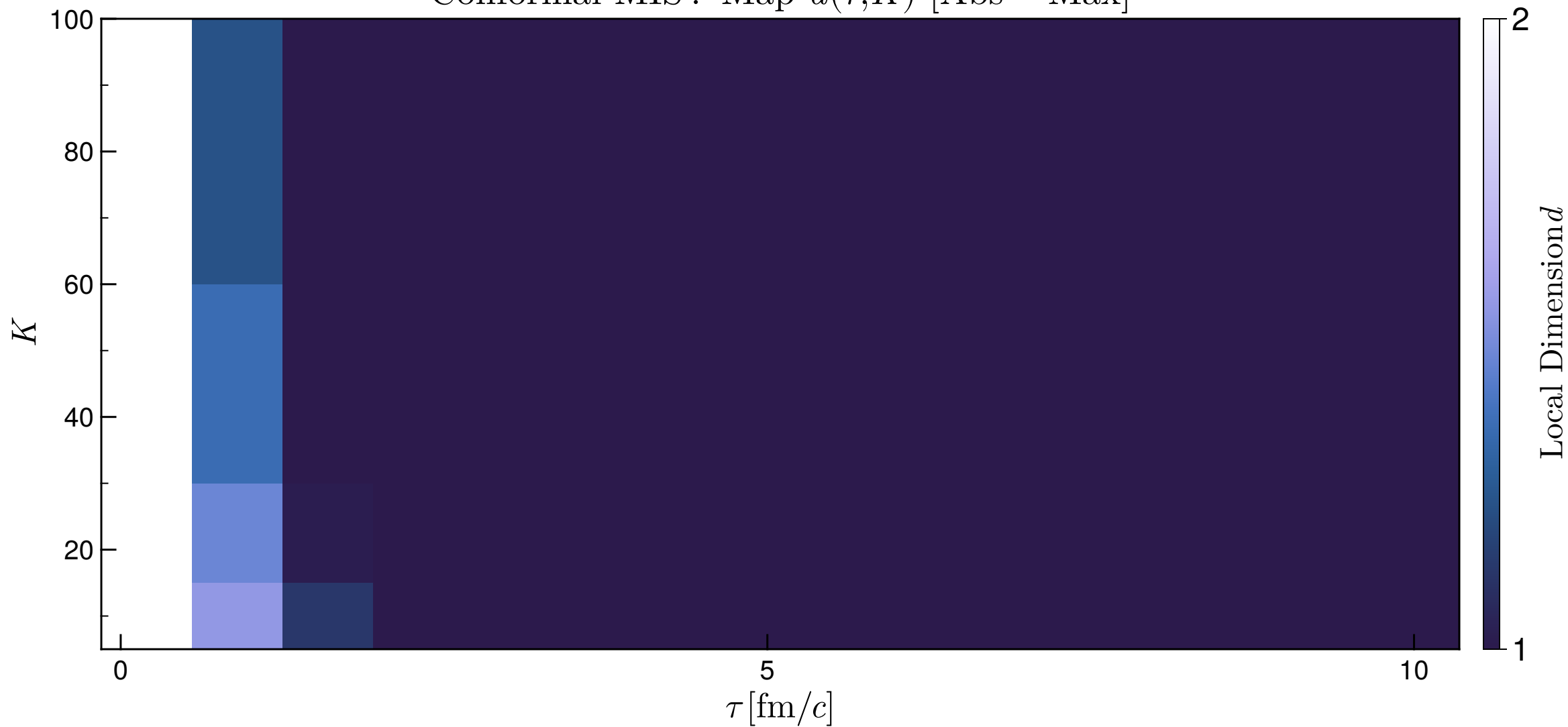
Conformal MIS : Map d(\tau, K) [Abs - Max]
