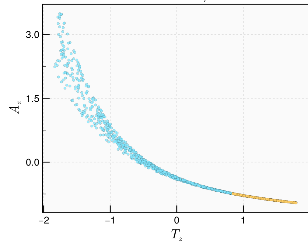
\tau = 2.5 \text{ fm}/c
