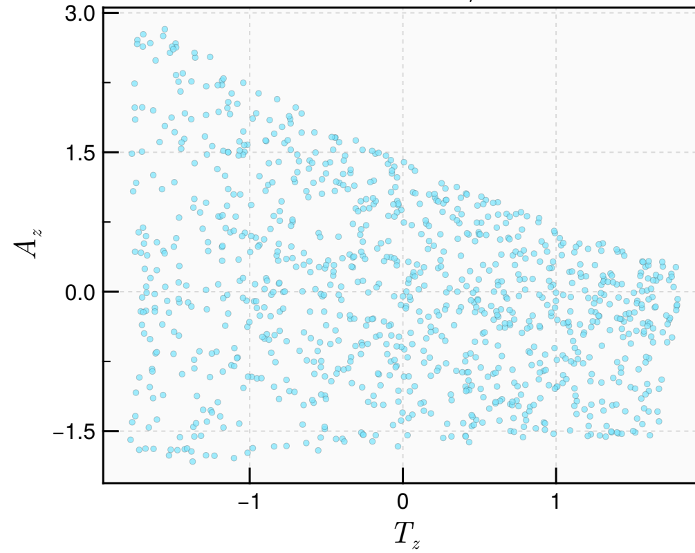
\tau = 0.55 \text{ fm}/c
