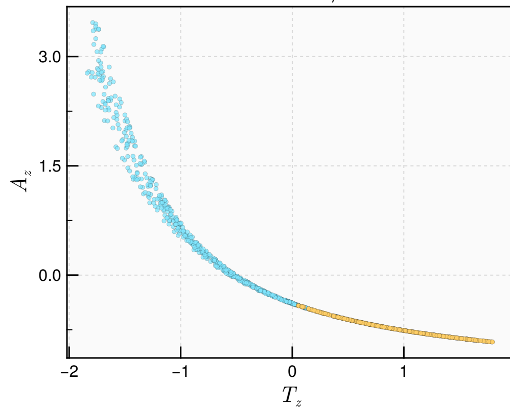
\tau = 0.8 \text{ fm}/c
