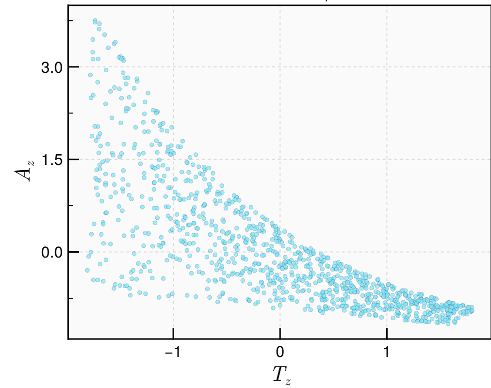
\tau = 0.65 \text{ fm}/c
