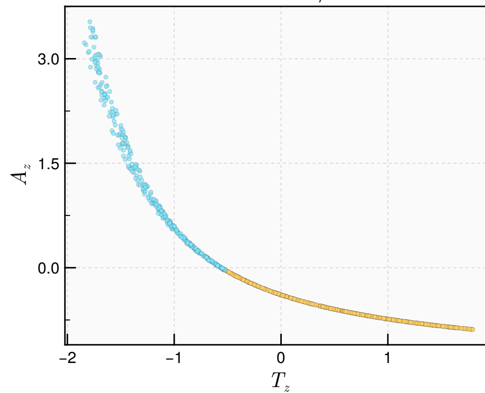
\tau = 1.0 \text{ fm}/c
