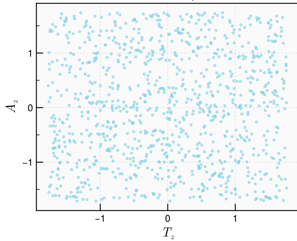
\tau = 0.45 \text{ fm}/c
