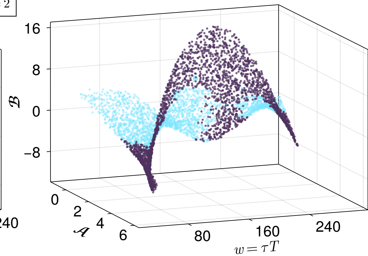
\tau = 0.65 \text{ fm}/c
