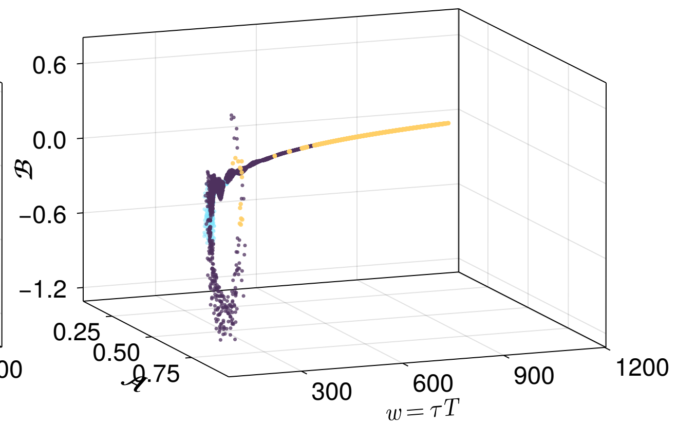
\tau = 2.5 \text{ fm}/c
