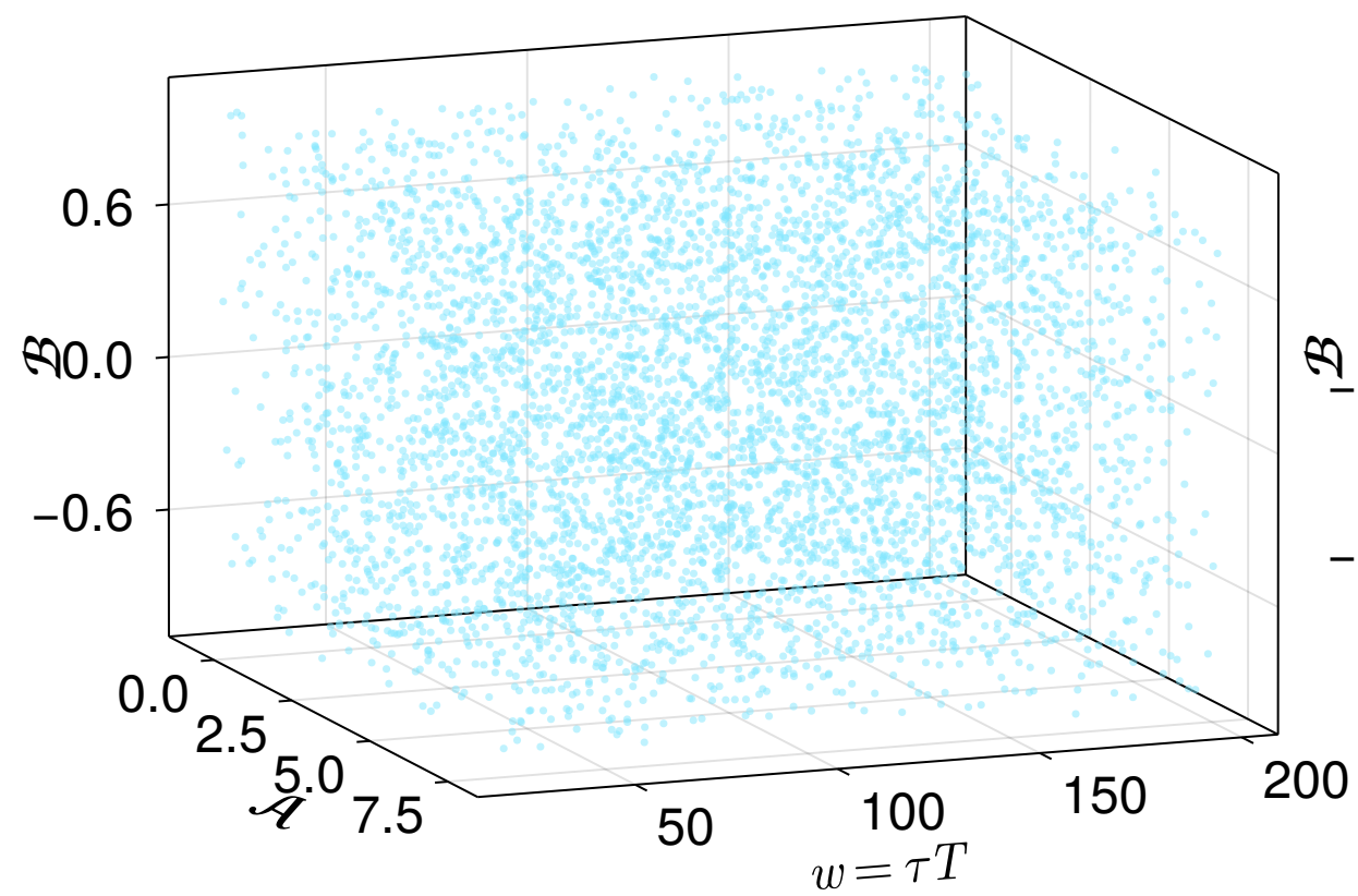
\tau = 0.45 \text{ fm}/c
