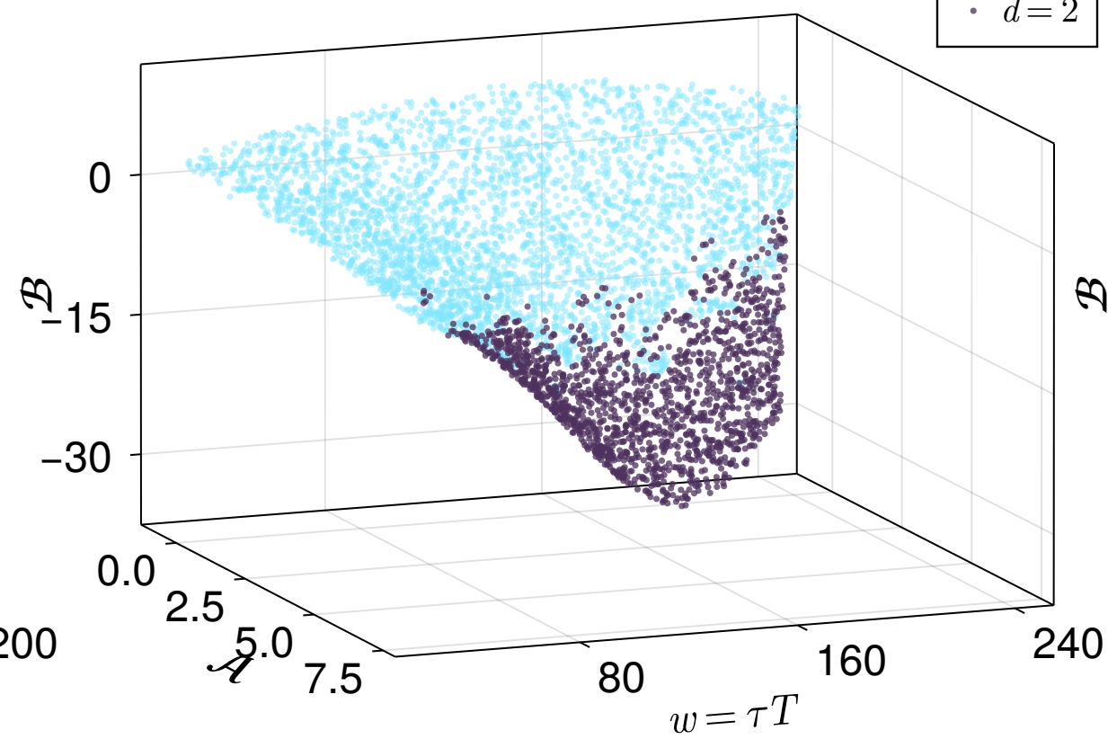
\tau = 0.55 \text{ fm}/c
