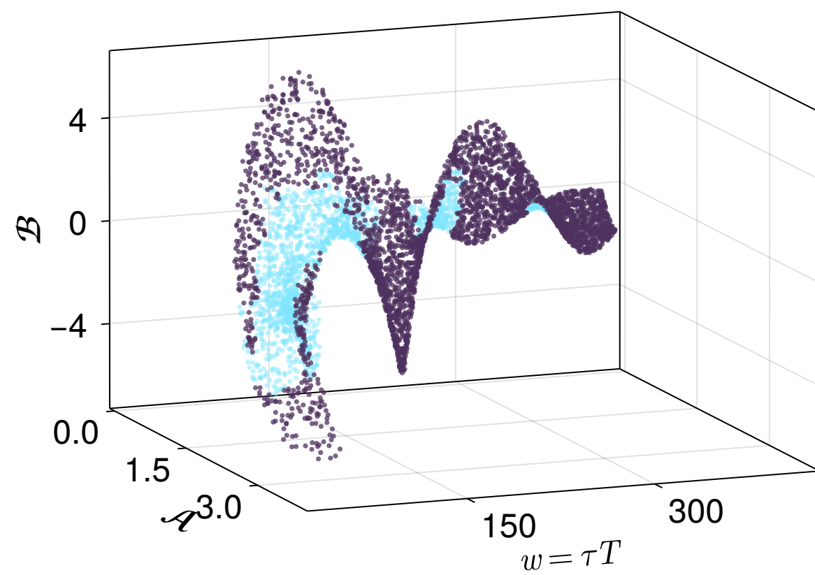
\tau = 1.0 \text{ fm}/c
