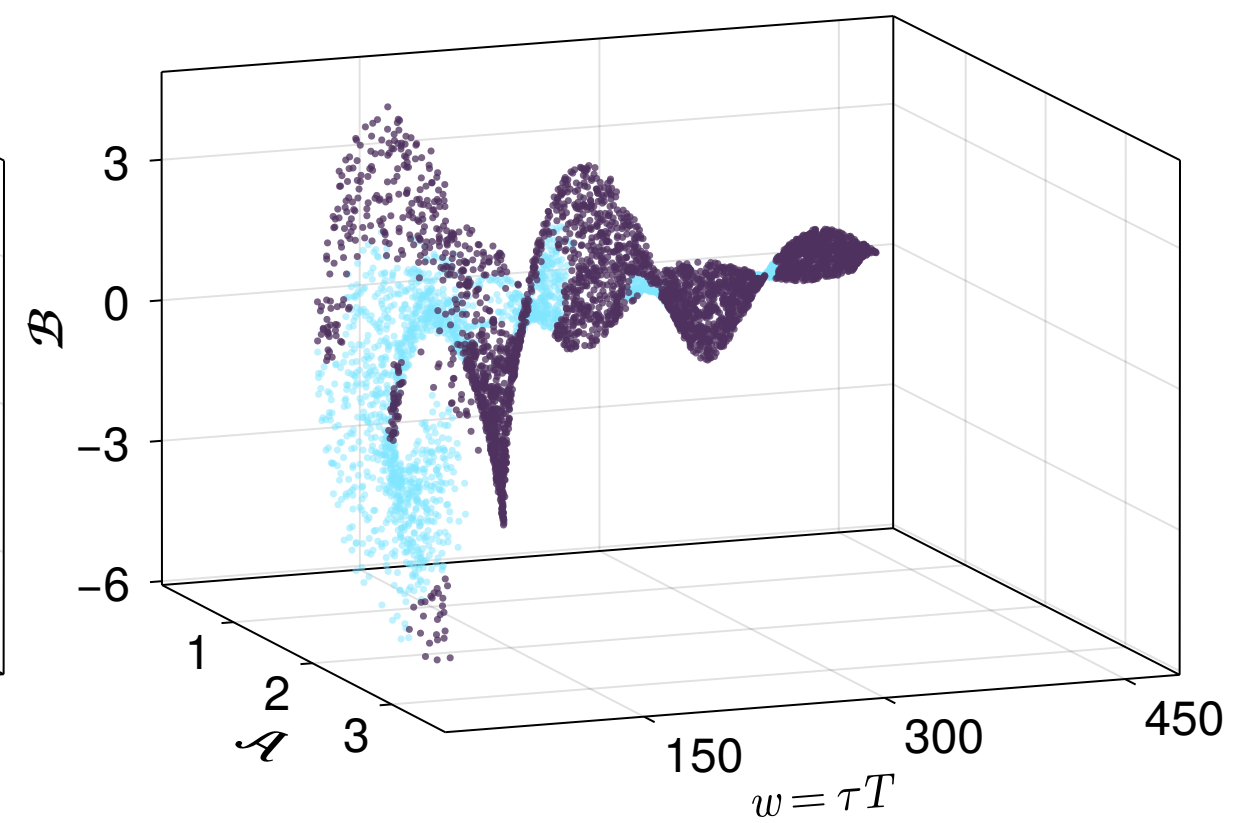
\tau = 2.5 \text{ fm}/c
