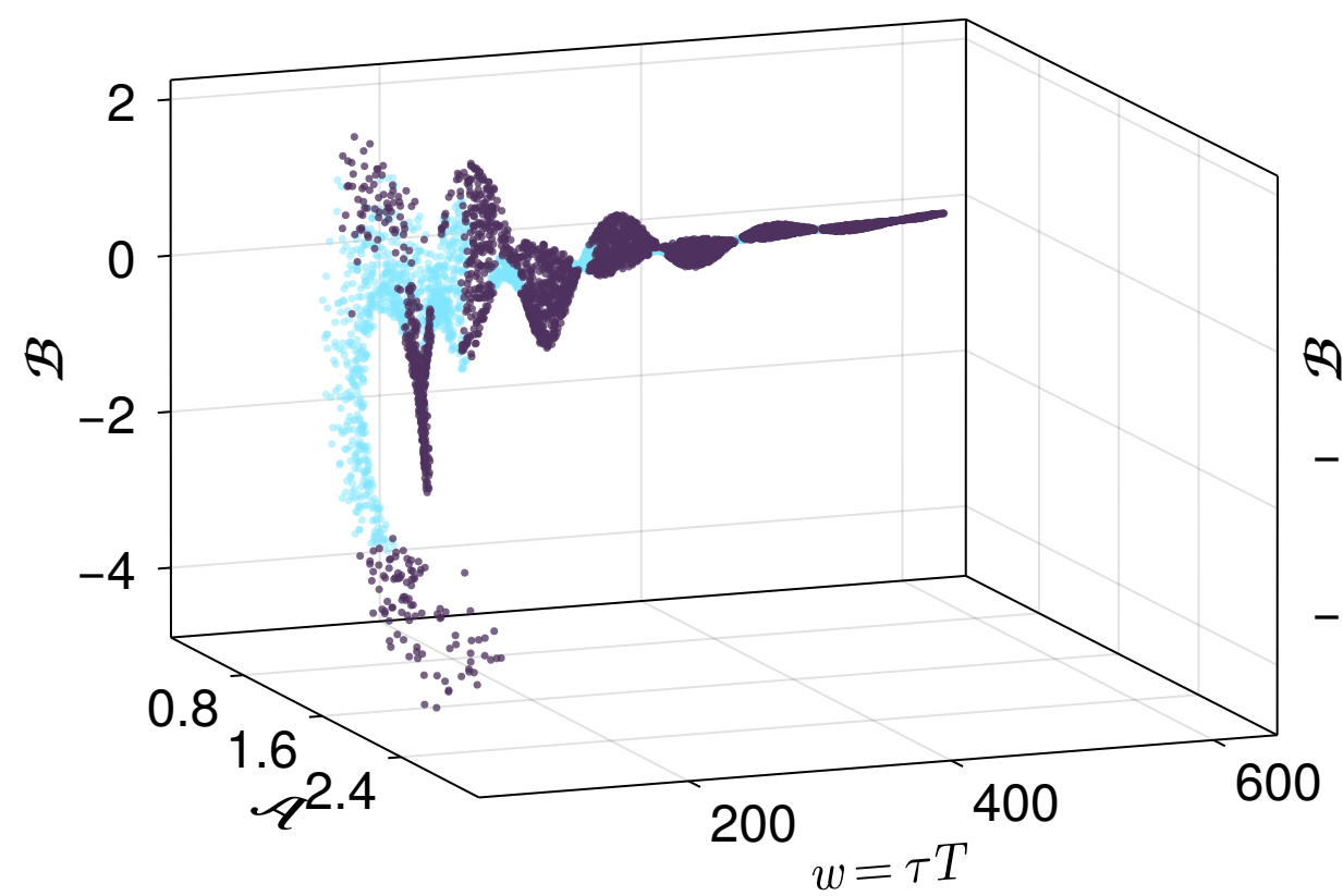
\tau = 1.0 \text{ fm}/c
