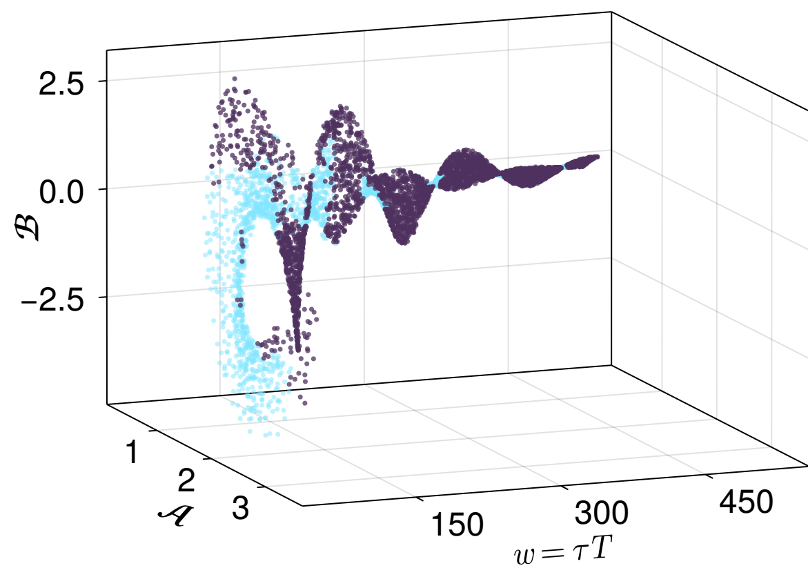
\tau = 0.8 \text{ fm}/c
