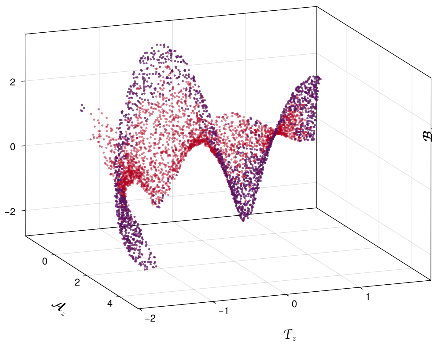
\tau = 0.8 \text{ fm}/c
