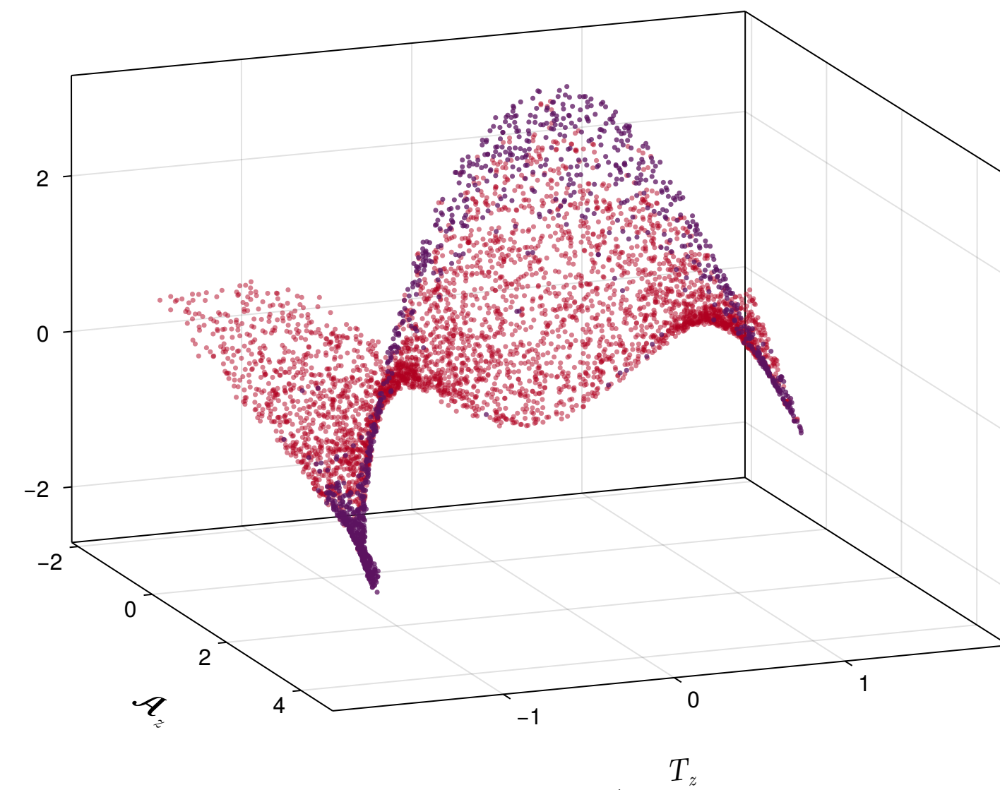
\tau = 0.35 \text{ fm}/c
