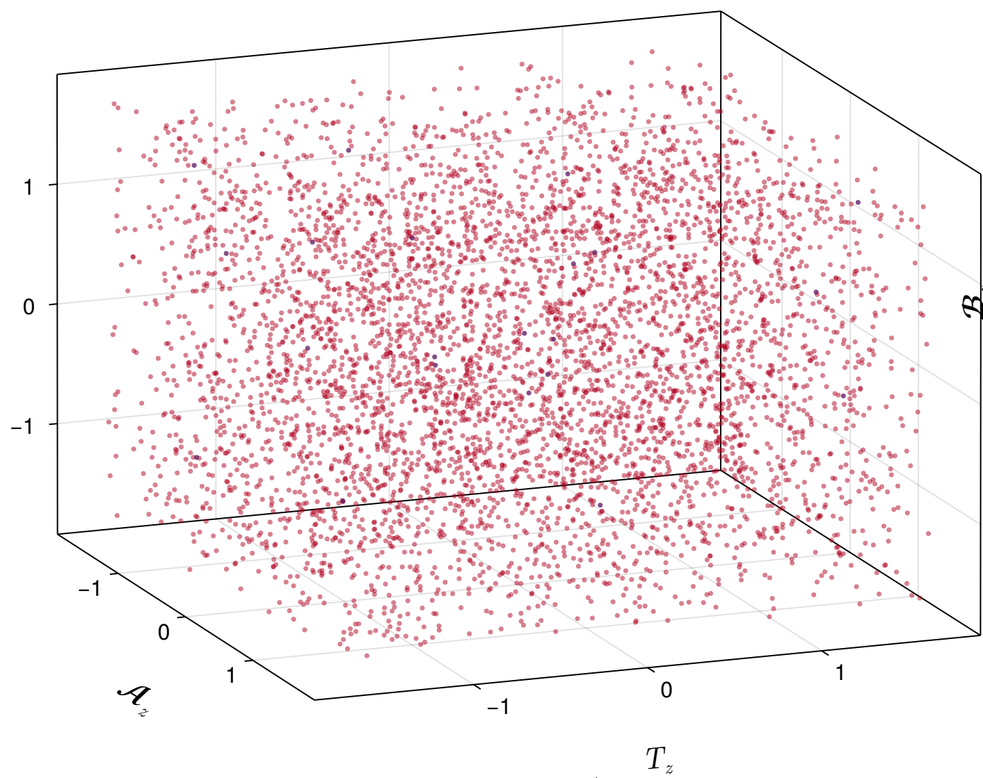
\tau = 0.2 \text{ fm}/c
