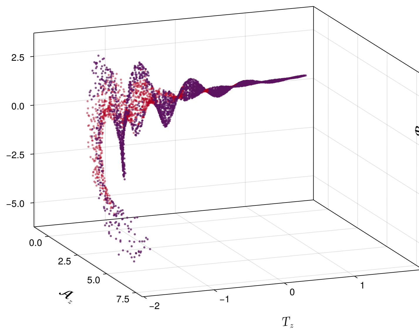
\tau = 1.0 \text{ fm}/c
