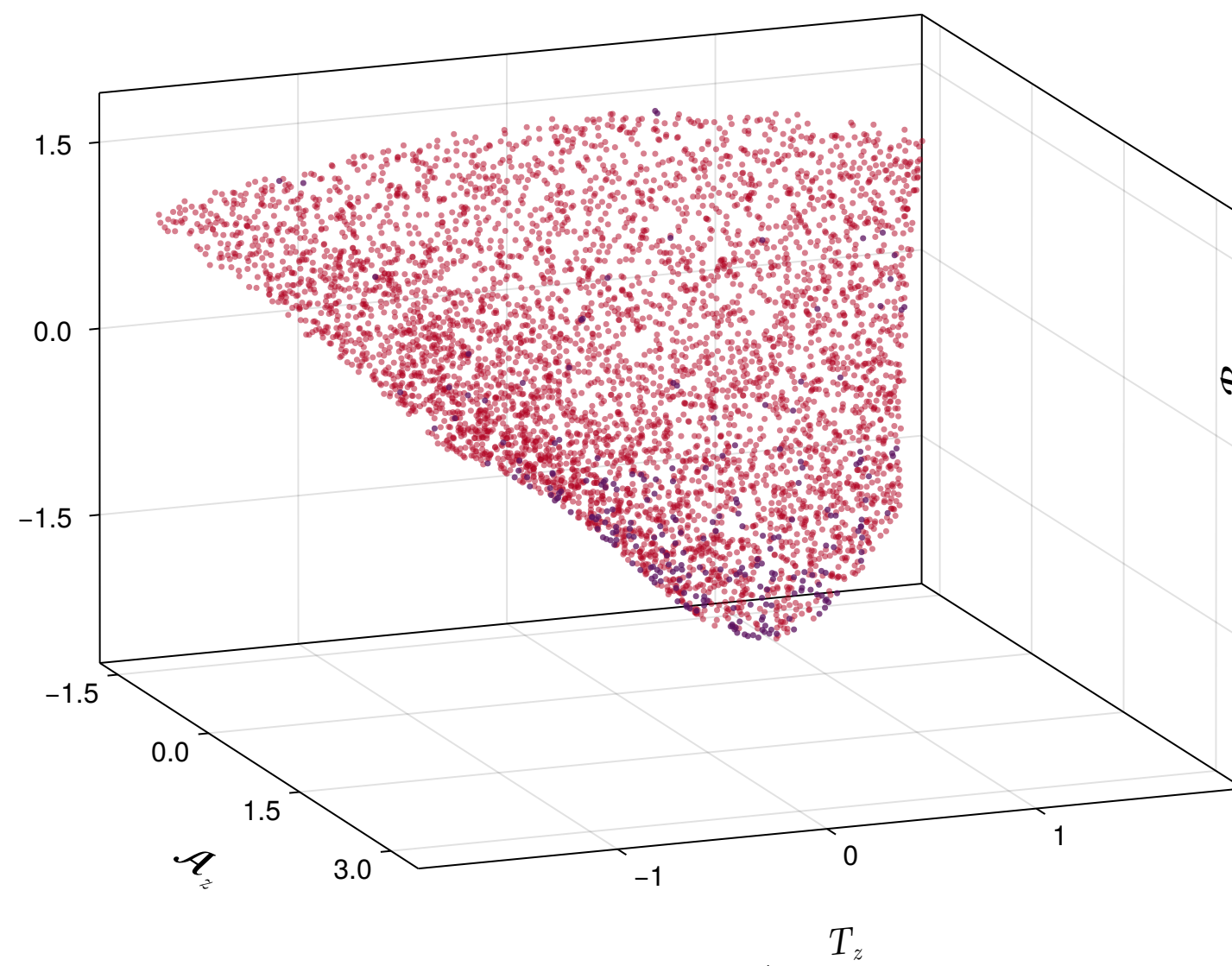
\tau = 0.25 \text{ fm}/c
