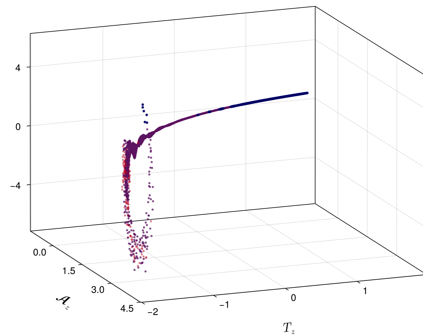
\tau = 2.5 \text{ fm}/c
