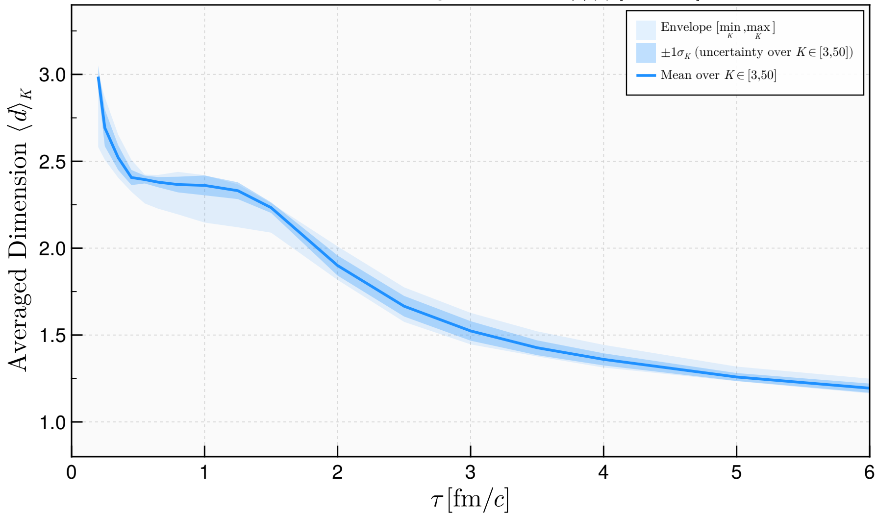
HJSW Model : K -Averaged Hard LPCA \langle d \rangle(\tau) [Z - Score]
