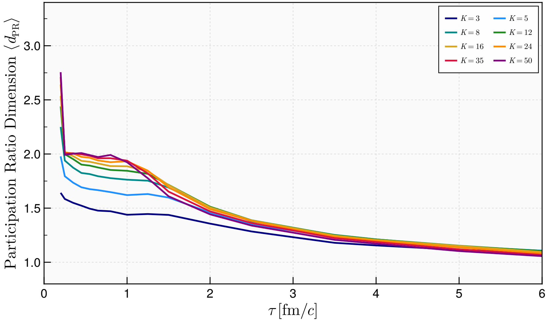
HJSW Model: Participation Ratio \langle d_{\text{PR}} \rangle(\tau) for varied K [Z-Score, Lines Only]
