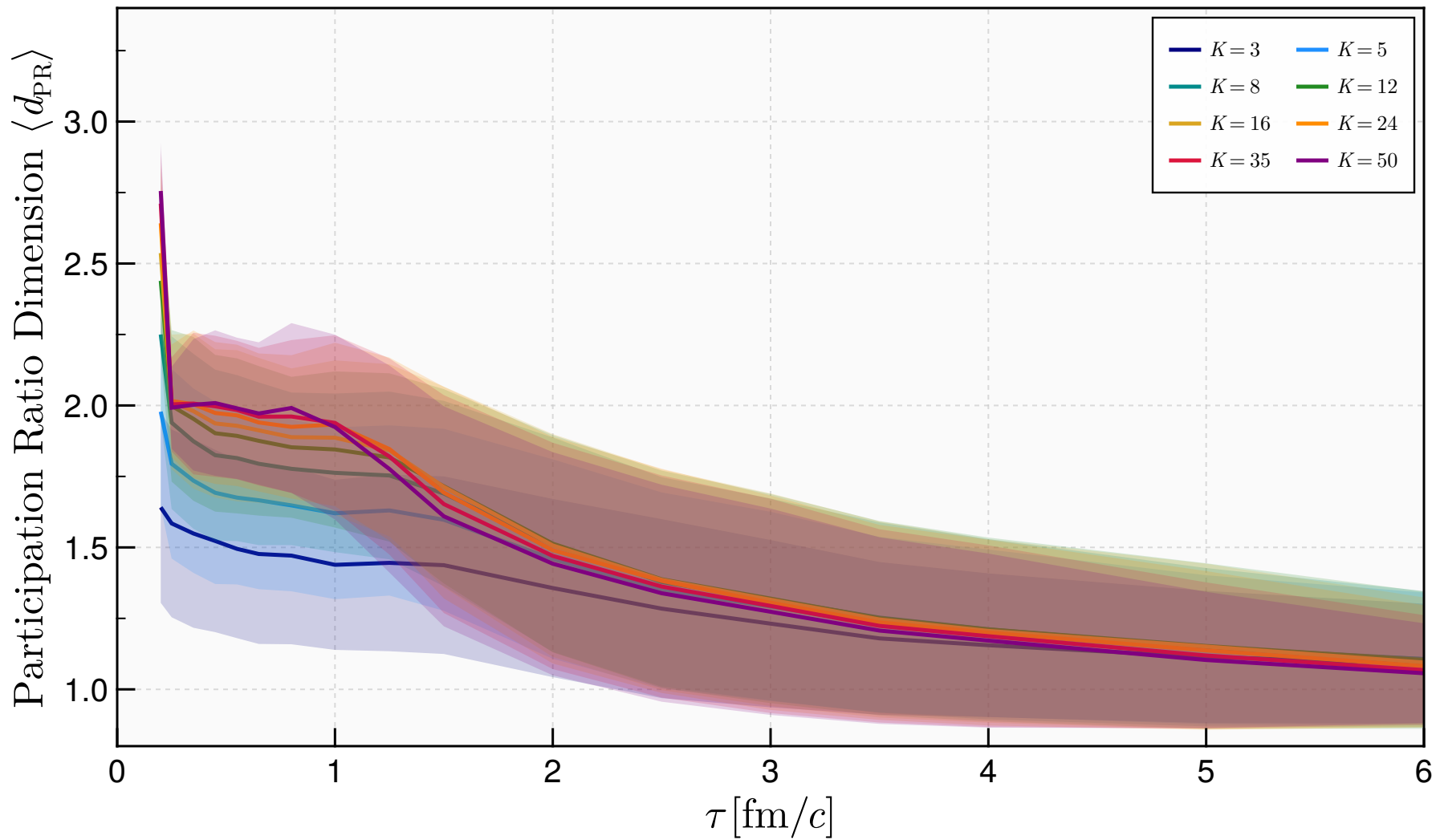
HJSW Model: Participation Ratio \langle d_{\text{PR}} \rangle(\tau) for varied K [Z - Score]
