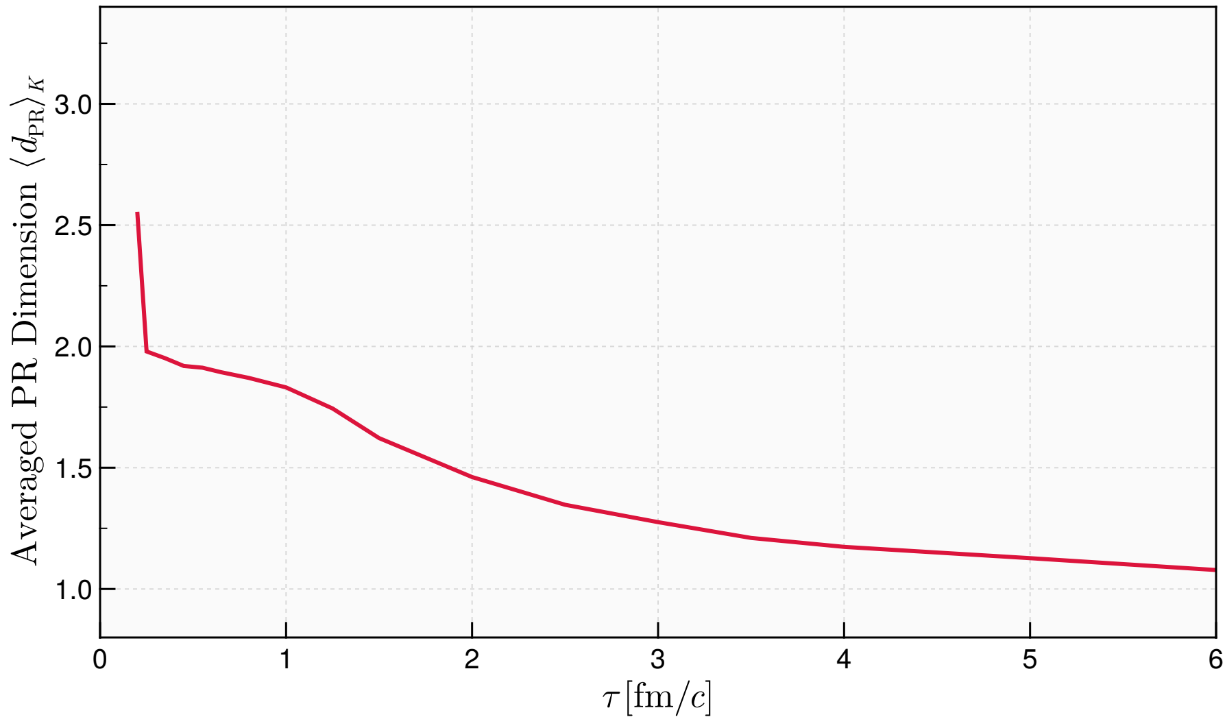
HJSW Model: K -Averaged Participation Ratio \langle d_{\text{PR}} \rangle_K(\tau) [Physical, Line Only]
