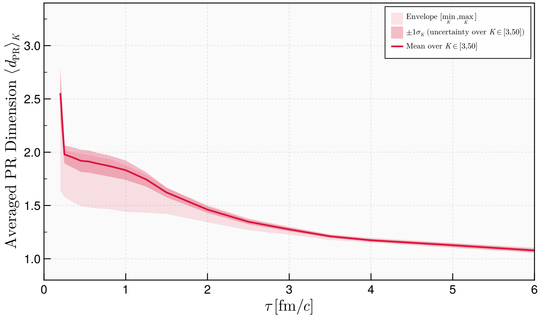
HJSW Model: K -Averaged Participation Ratio \langle d_{\text{PR}} \rangle_K(\tau) [Physical (T, \mathcal{A}, \mathcal{B}) ]
