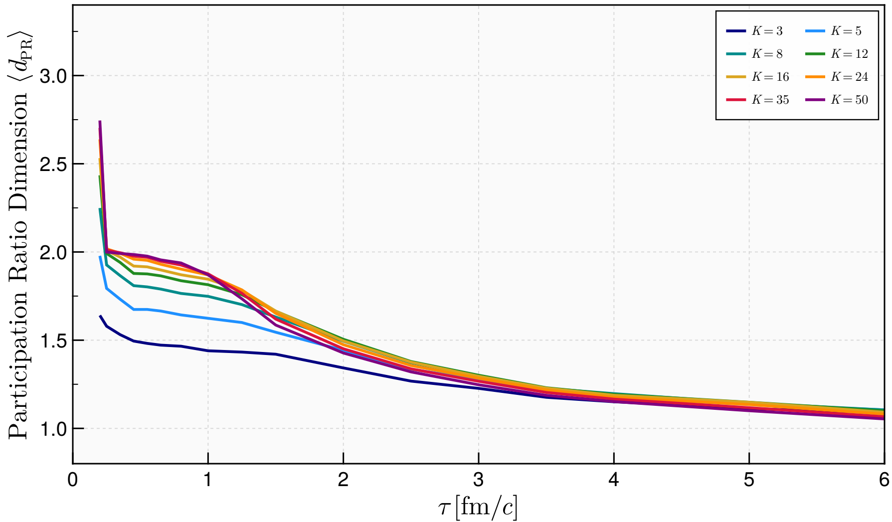
HJSW Model: Participation Ratio \langle d_{\text{PR}} \rangle(\tau) for varied K [Physical, Lines Only]
