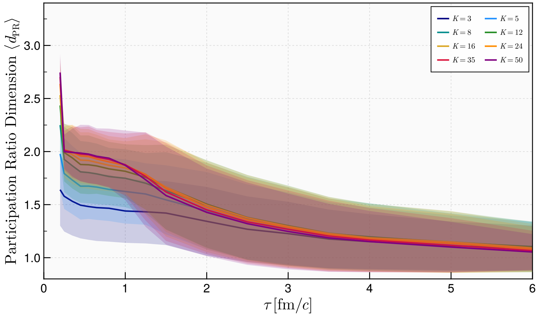
HJSW Model: Participation Ratio \langle d_{\text{PR}} \rangle(\tau) for varied K [Physical (T, \mathcal{A}, \mathcal{B}) ]
