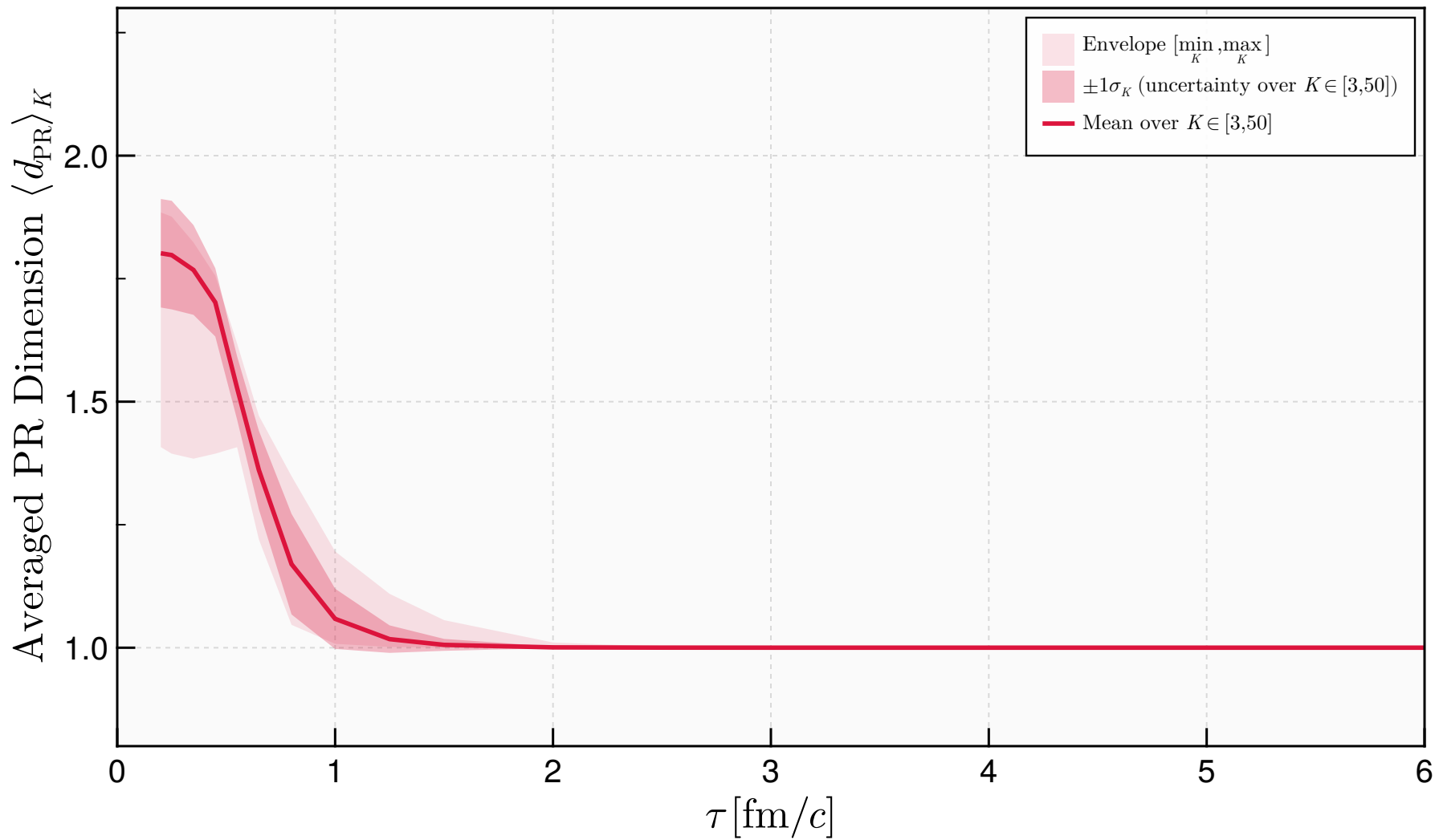
Conformal MIS : K -Averaged Participation Ratio \langle d_{\text{PR}} \rangle(\tau) [Z - Score]
