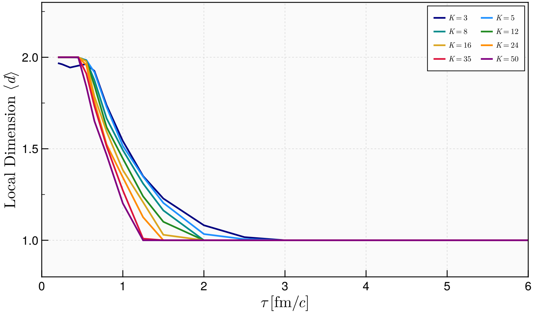
Conformal MIS: Hard LPCA \langle d \rangle(\tau) for varied K [Z-Score, Lines Only]
