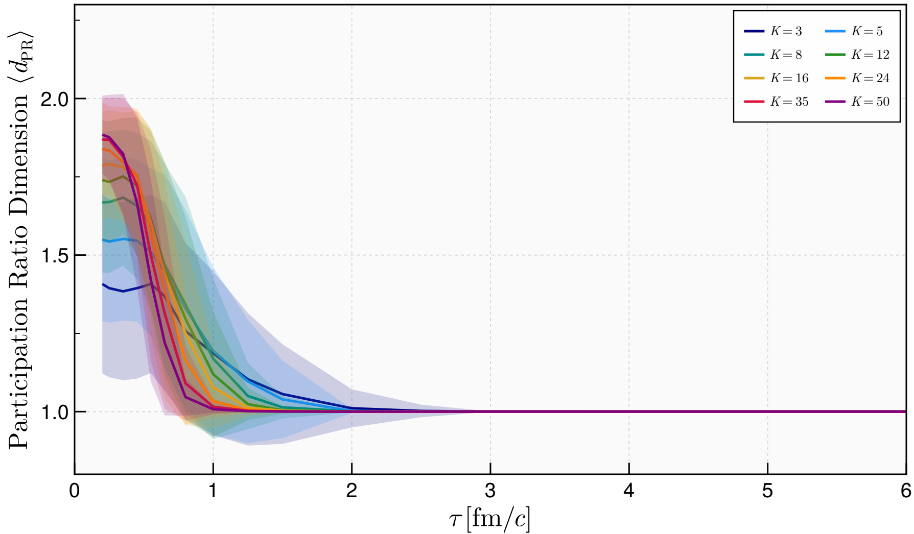
Conformal MIS: Participation Ratio \langle d_{\text{PR}} \rangle(\tau) for varied K [Z-Score]
