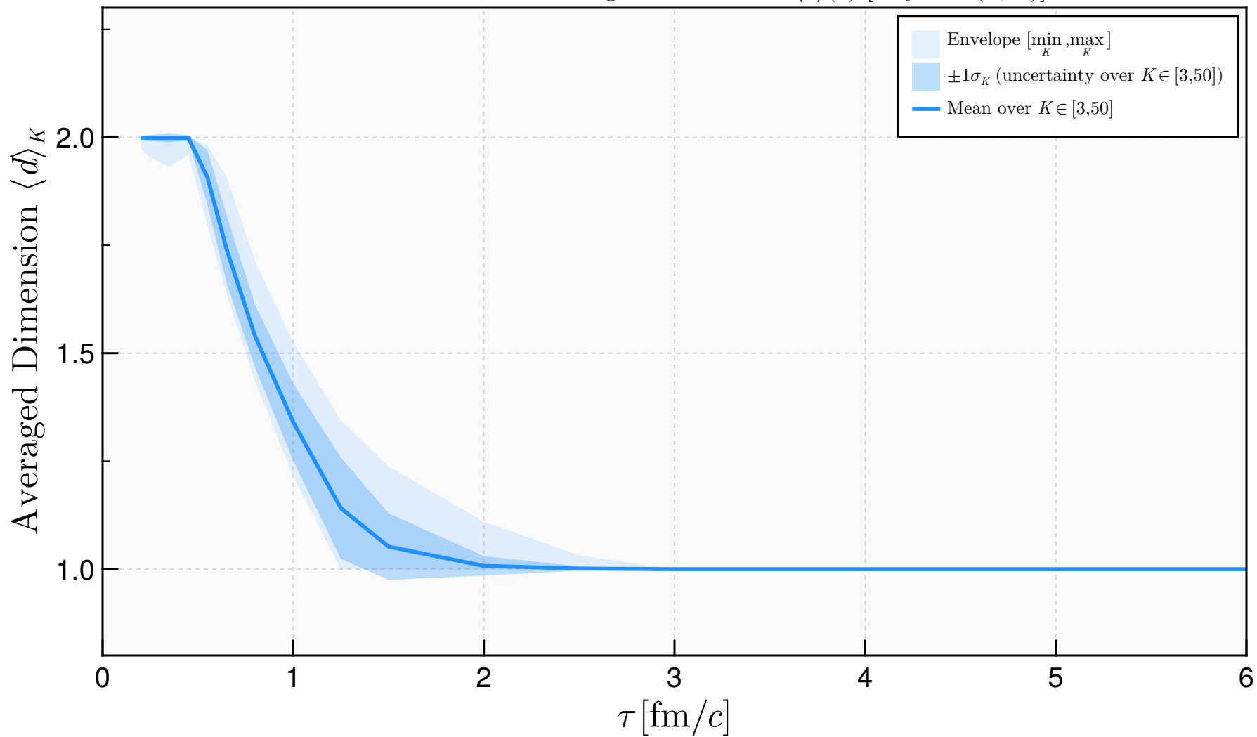
Conformal MIS : K -Averaged Hard LPCA \langle d \rangle(\tau) [Physical (T, \mathcal{A}) ]
