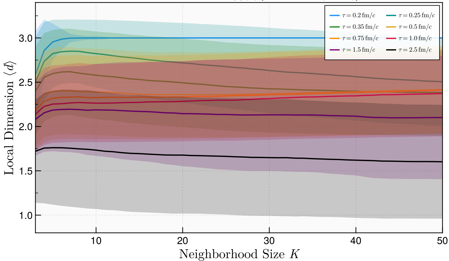
HJSW Model: Hard LPCA \langle d \rangle(K) [Dimensionless (w, \mathcal{A}, \mathcal{B}) ]
