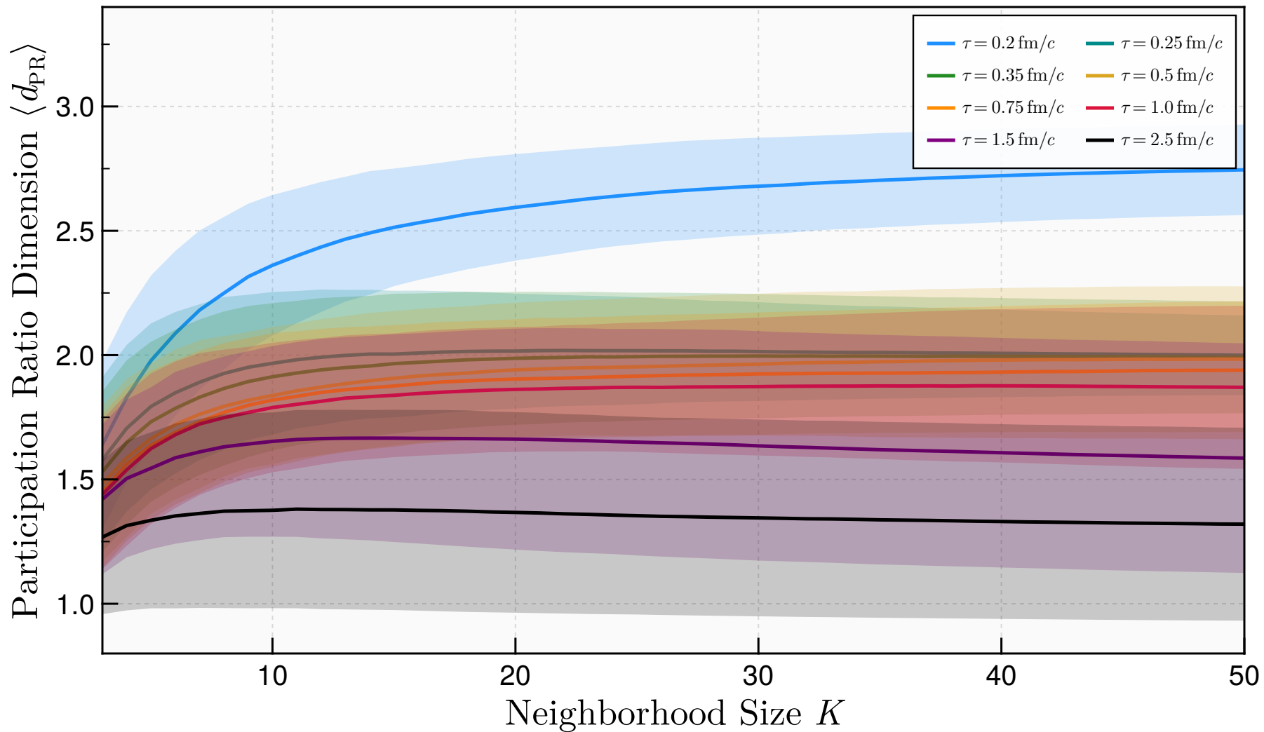
HJSW Model: Participation Ratio \langle d_{\text{PR}} \rangle(K) [Dimensionless ( w, \mathcal{A}, \mathcal{B} )]
