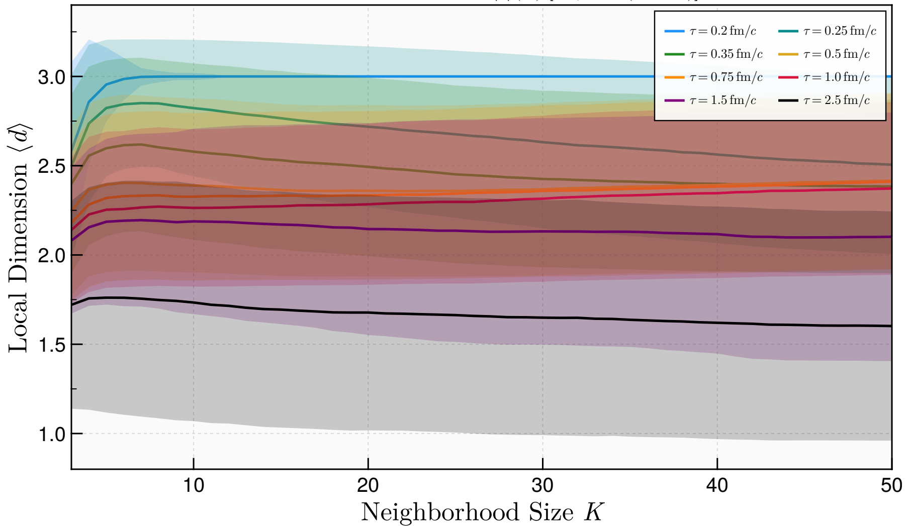
HJSW Model: Hard LPCA \langle d \rangle(K) [Physical (T, \mathcal{A}, \mathcal{B}) ]
