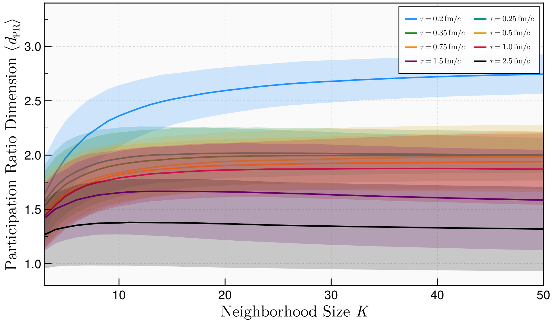
HJSW Model: Participation Ratio \langle d_{\text{PR}} \rangle(K) [Physical (T, \mathcal{A}, \mathcal{B}) ]
