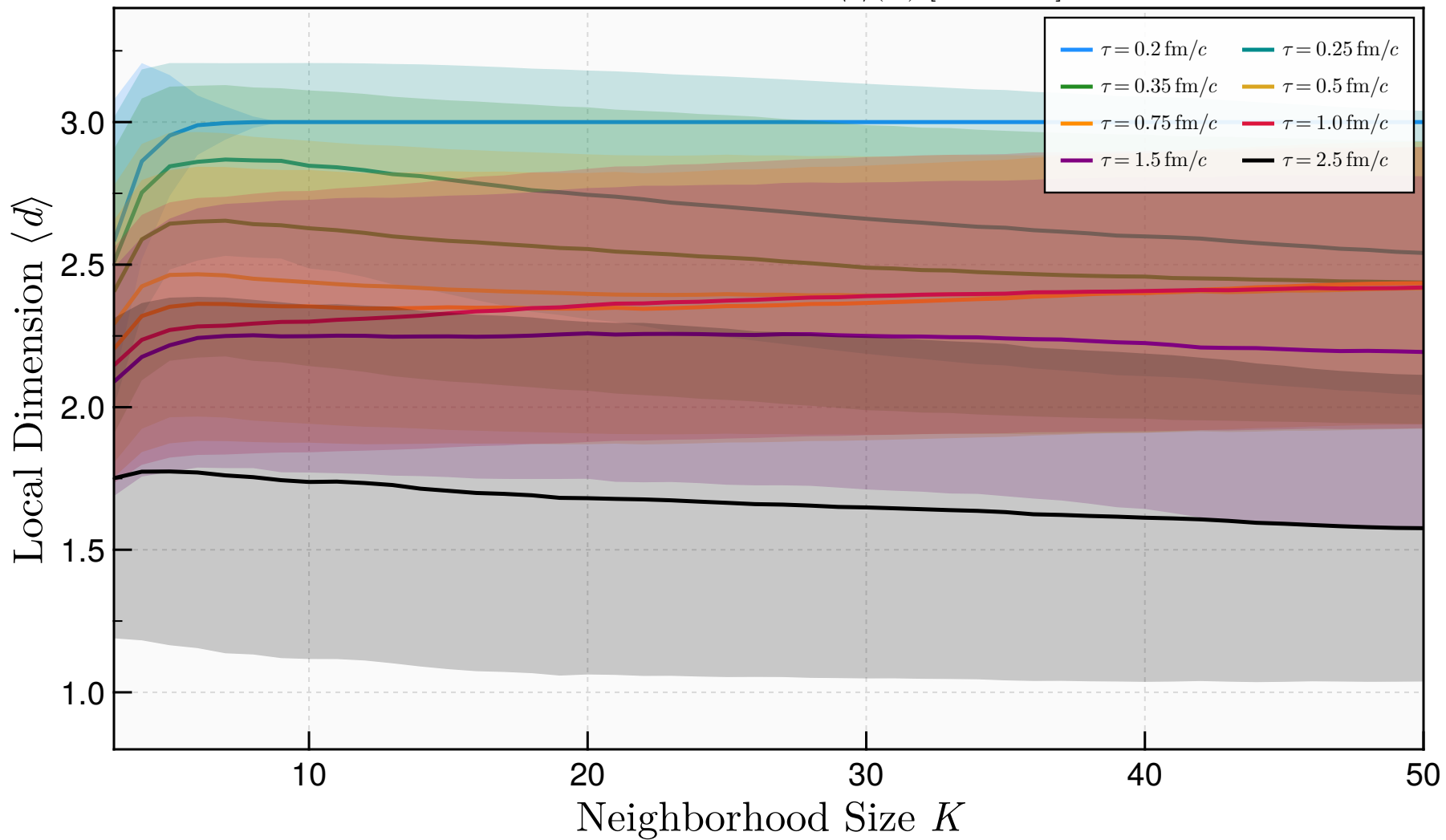
HJSW Model: Hard LPCA \langle d \rangle(K) [Z - Score]
