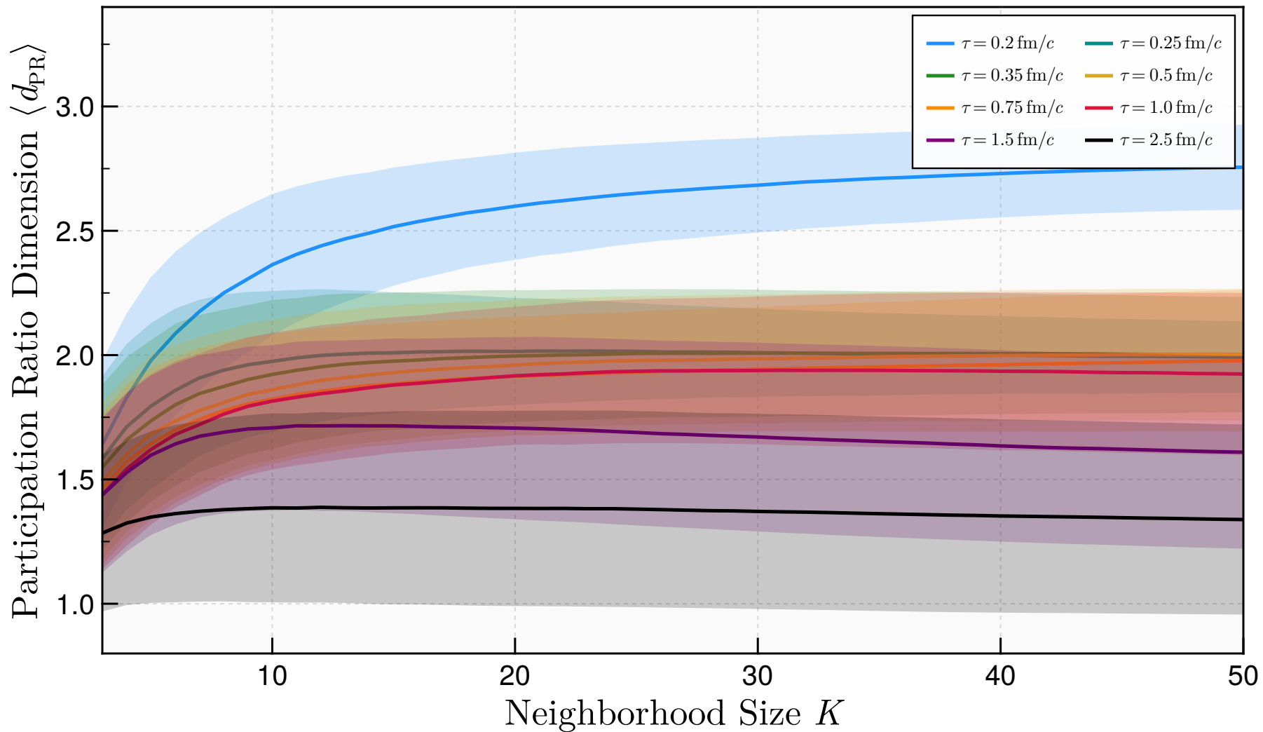
HJSW Model: Participation Ratio \langle d_{\text{PR}} \rangle(K) [Z-Score]
