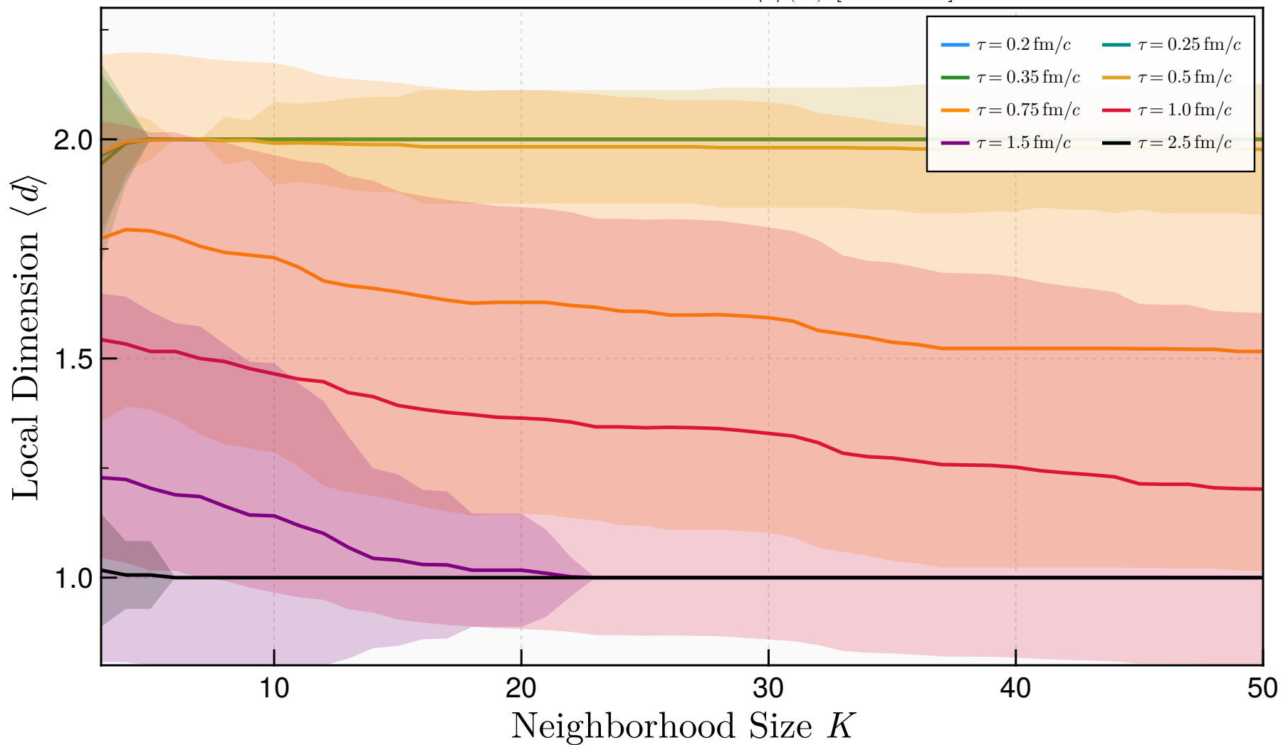
Conformal MIS: Hard LPCA \langle d \rangle(K) [Z - Score]
