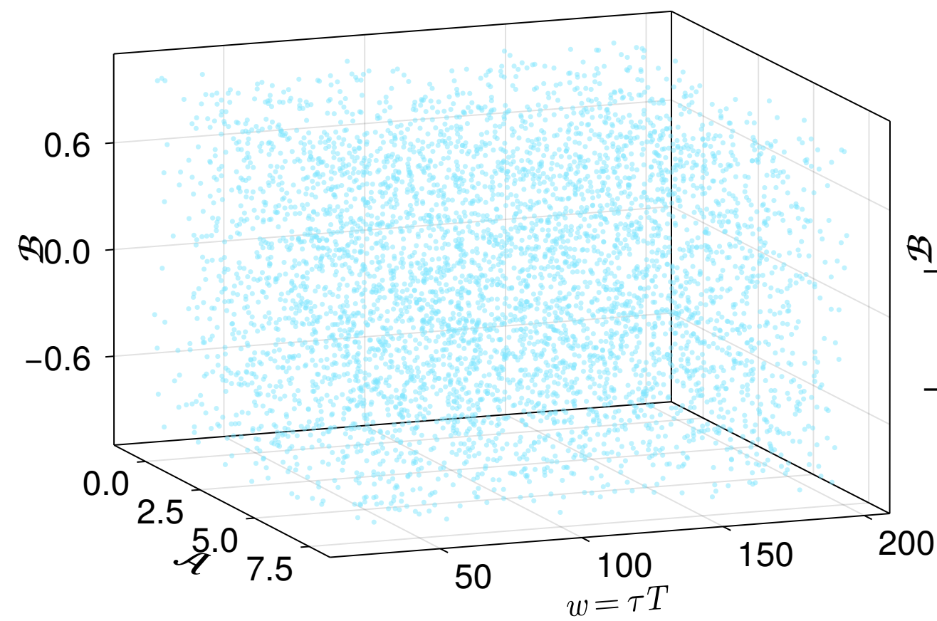
\tau = 0.45 \text{ fm}/c
