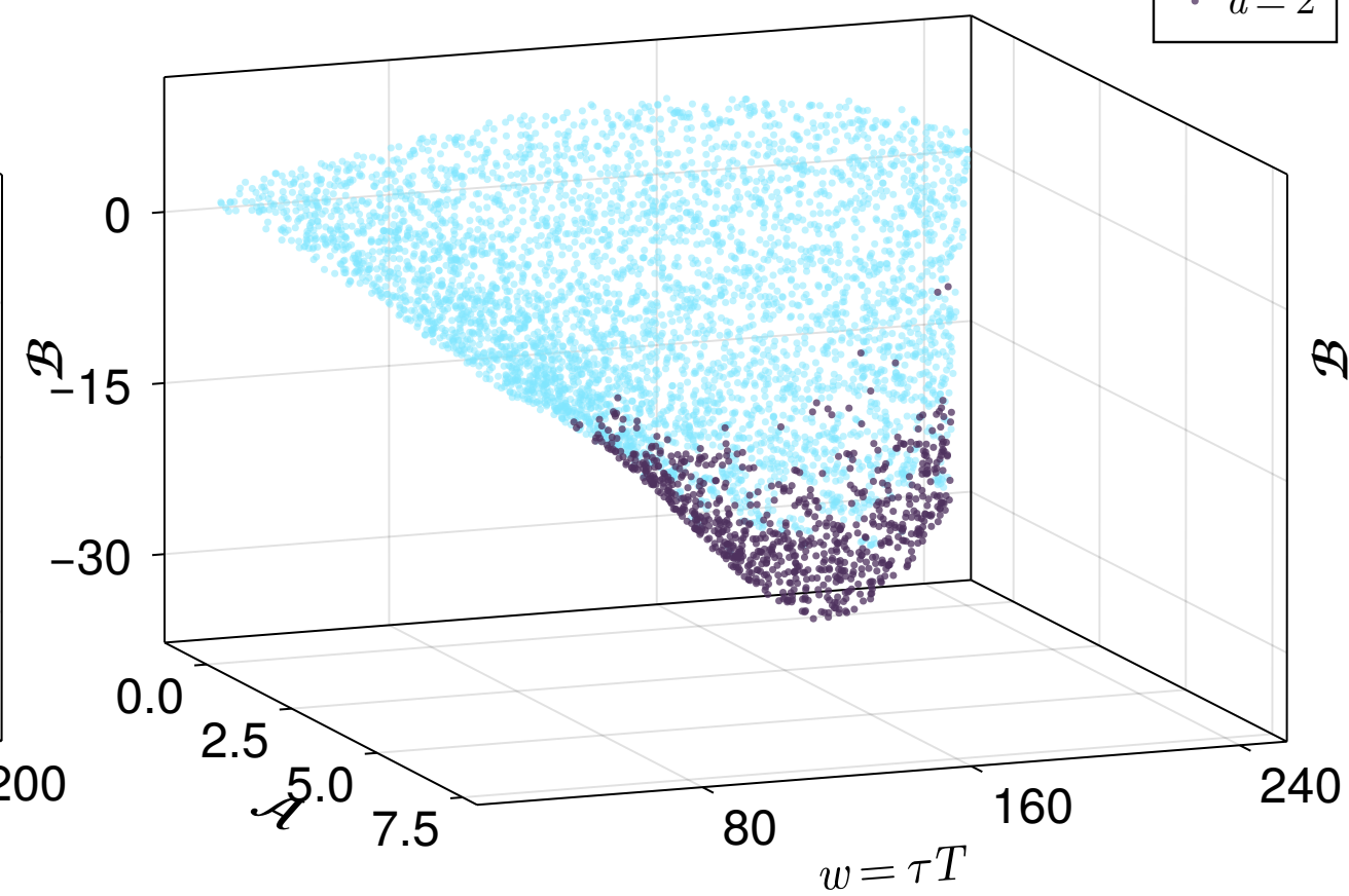
\tau = 0.55 \text{ fm}/c
