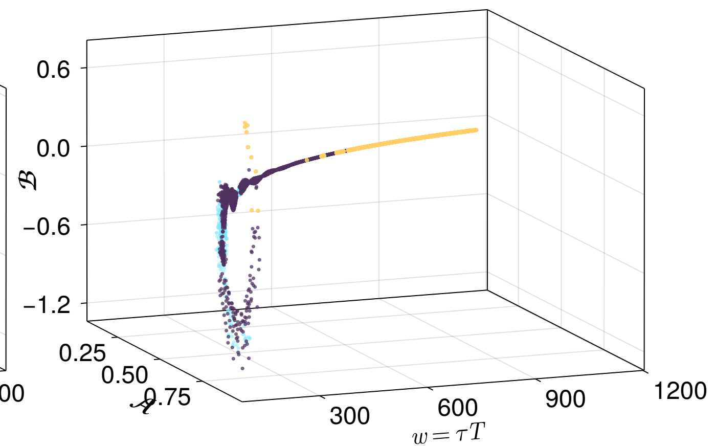
\tau = 2.5 \text{ fm}/c
