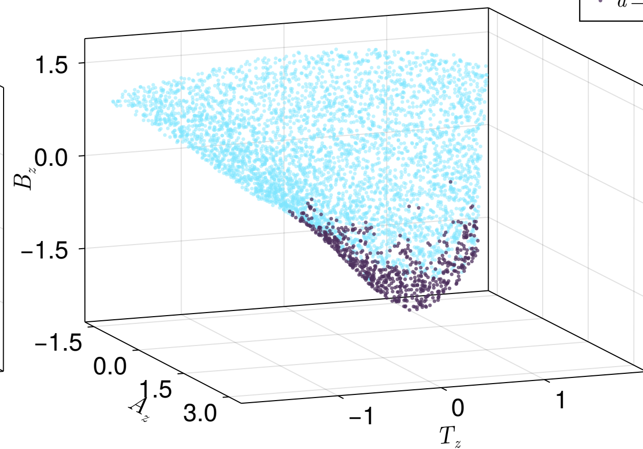
\tau = 0.55 \text{ fm}/c
