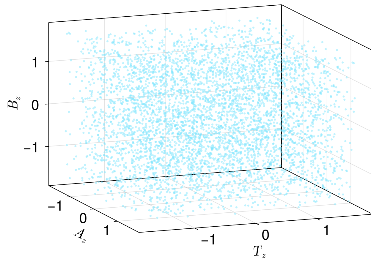
\tau = 0.45 \text{ fm}/c
