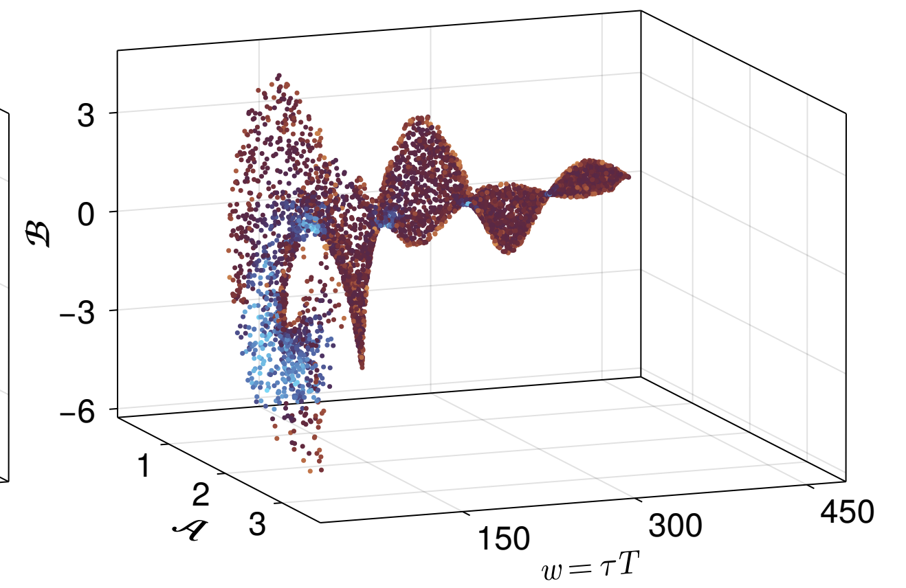
\tau = 2.5 \text{ fm}/c
