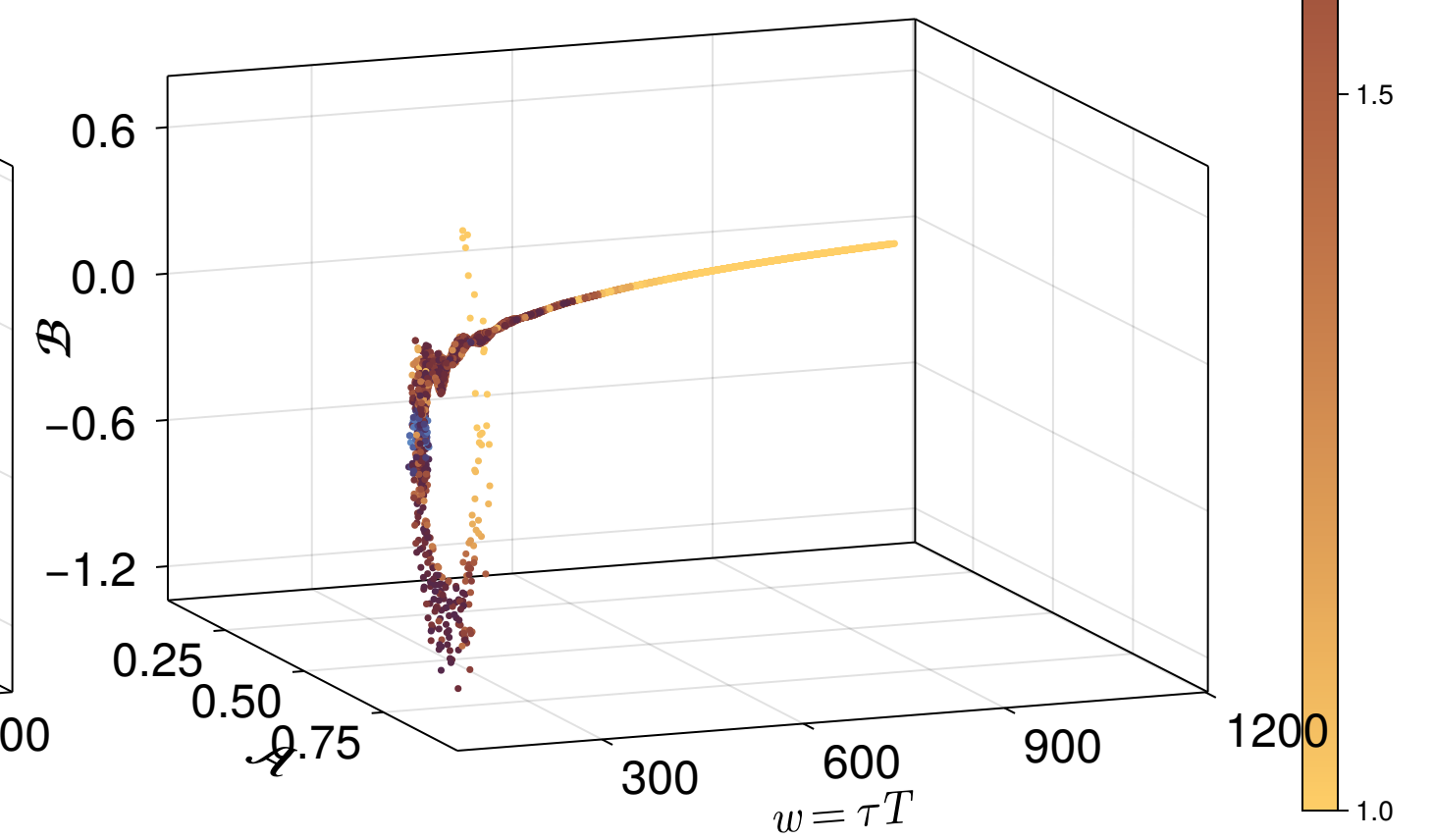
\tau = 2.5 \text{ fm}/c
