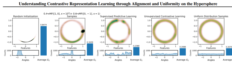
Figure 4: Average pairwise G_2 potential as a measure of uniformity. Each plot shows 10000 points distributed on S^1 . The plots are generated via either applying an encoder on CIFAR-10 validation set (same as those in Figure 3) or sampling from uniform distribution on S^1 , as described in plot titles. We show the points with Gaussian KDE and the angles with vMF KDE.
