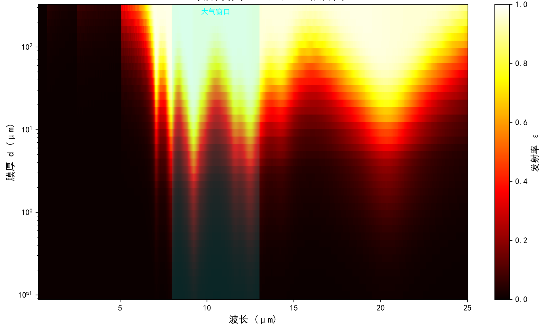
PDMS 薄膜发射率 \varepsilon(\lambda, d) 热力图
