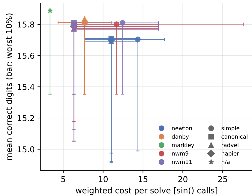
Cost vs accuracy (median cost, 10-90% range)
