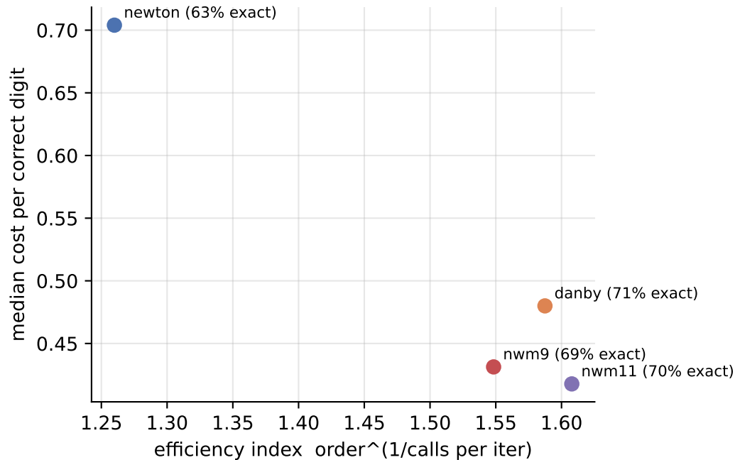
Generic index vs Kepler costing (no claimed order: markley)
