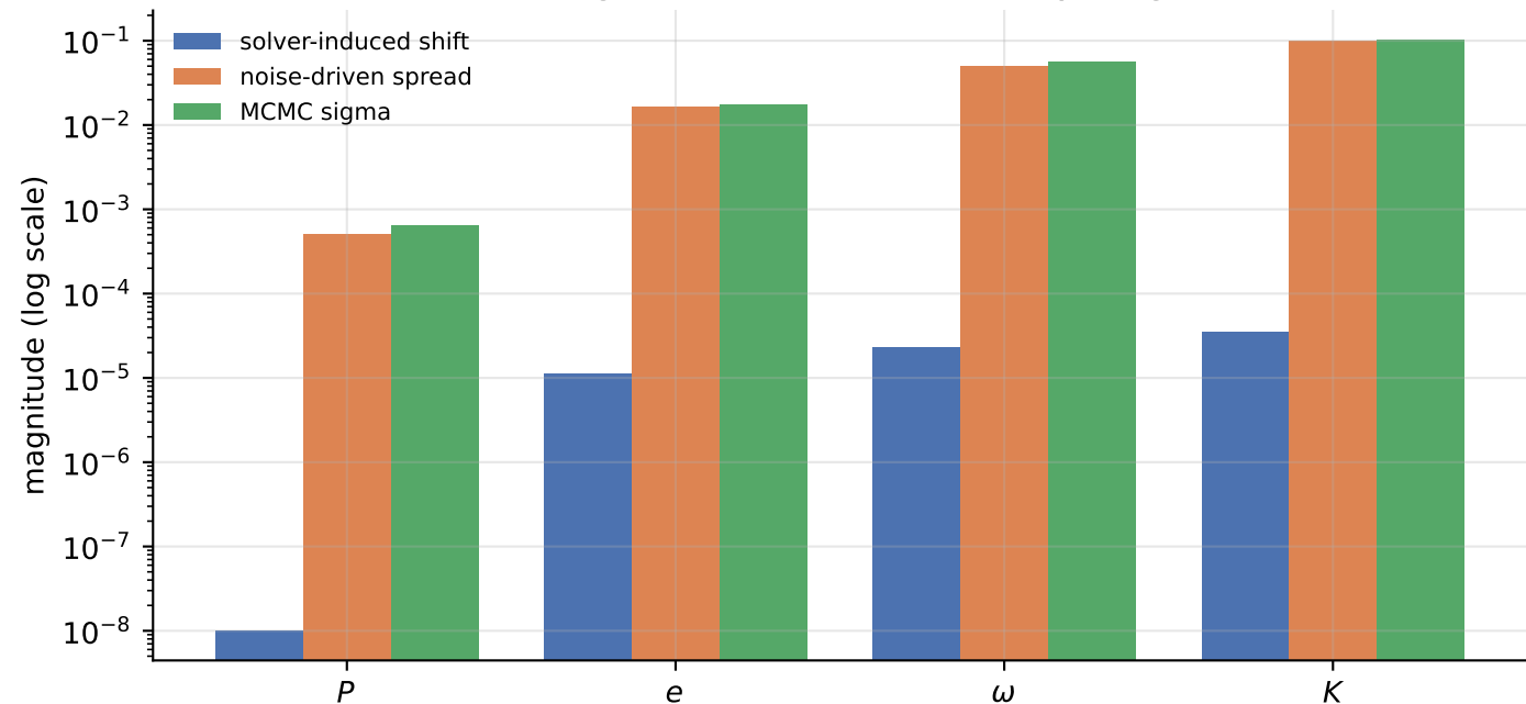
Error budget: solver choice vs. everything else
