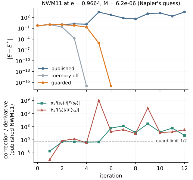
Figure 12: One repaired failure. Top: error per iteration for published, memory-off and guarded NWM11 at a hard-corner point. Bottom: the correction sizes the published method used. \beta_k ’s correction passes the guard’s limit at iterations 2 and 3 and reaches 10^9 at iteration 5, which throws the iterate about 3,000 radians away; the guarded version rejects those steps and converges in six iterations. Data: results/safeguard/trajectory.csv.
