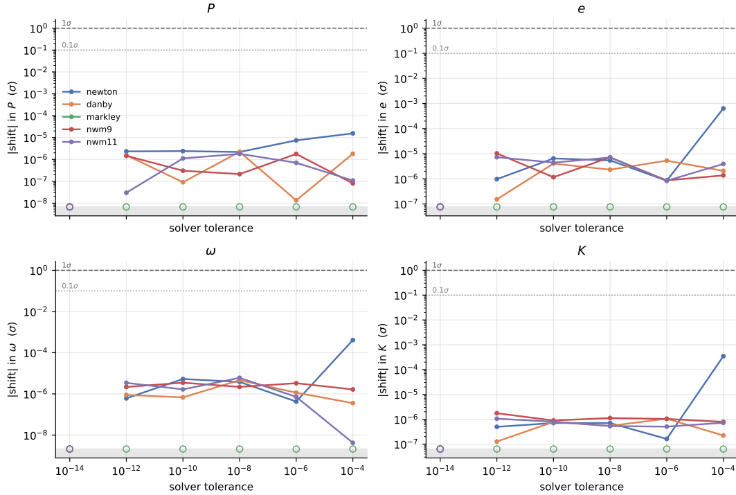
Figure 13: Parameter shift against solver tolerance, in units of the MCMC posterior width. Only Newton at 10^{-4} rises clearly above the floor set by the optimiser.
