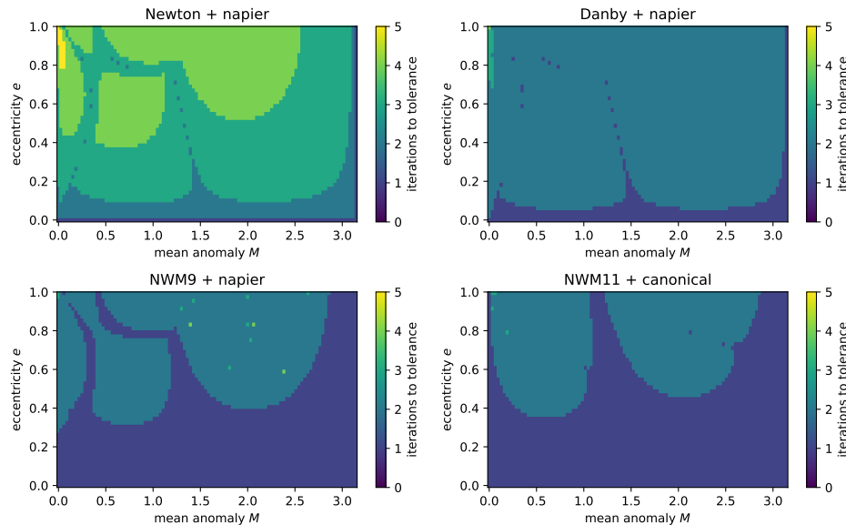
Figure 7: Iterations to tolerance on the even grid, each solver with its best guess. All four solvers are cheap almost everywhere; the cost is concentrated near e \rightarrow 1, M \rightarrow 0 .
