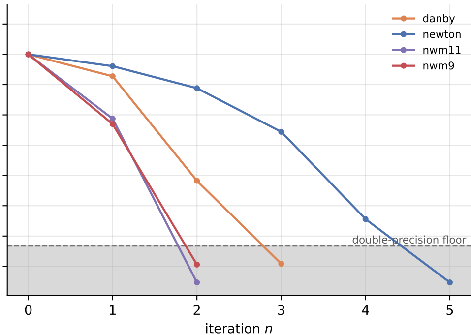
hard corner: e = 0.99 , M = 0.001
