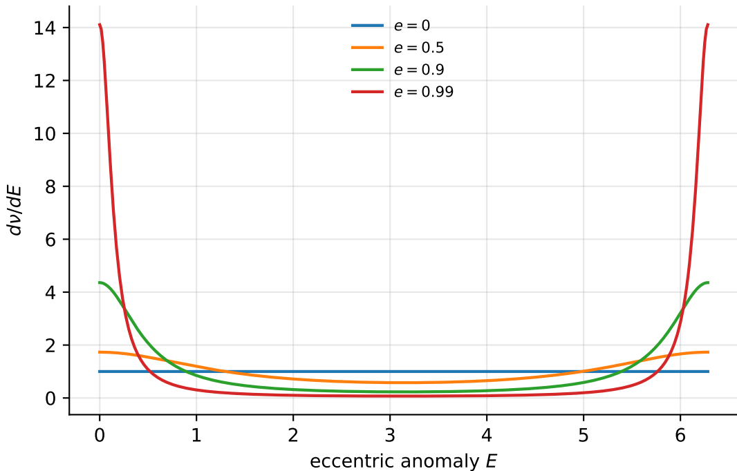
Error amplification from E into \nu
