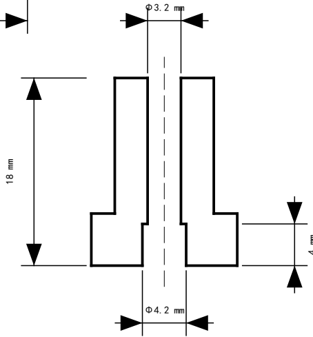
详图 C Detail C (2:1)
