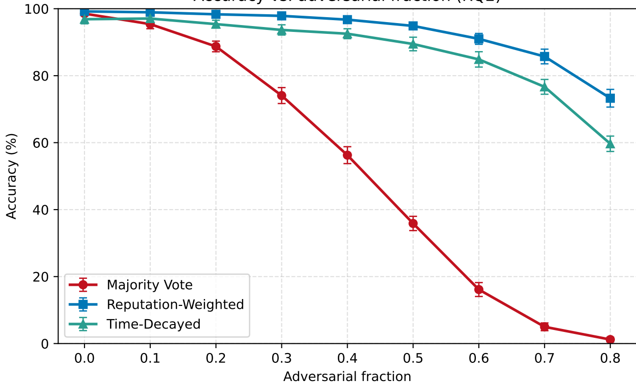
Accuracy vs. adversarial fraction (RQ2)
