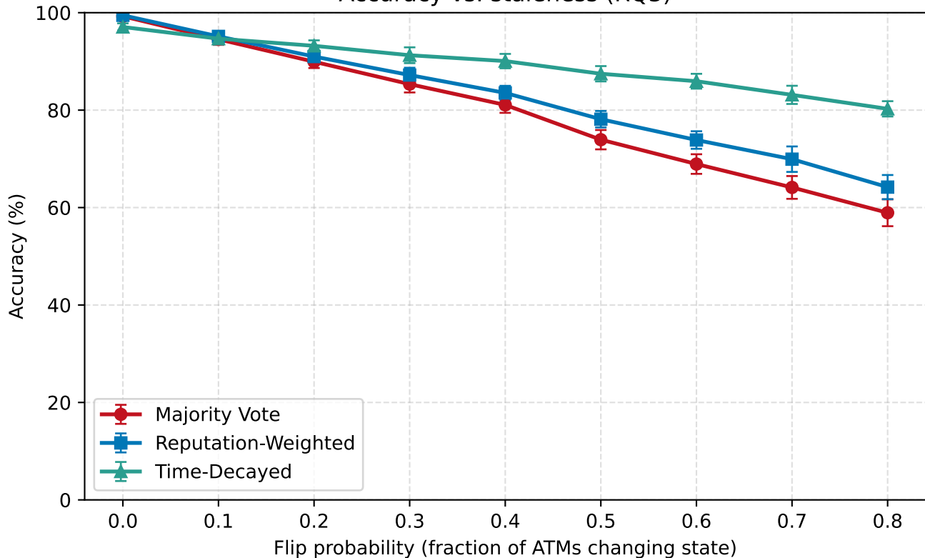
Accuracy vs. staleness (RQ3)
