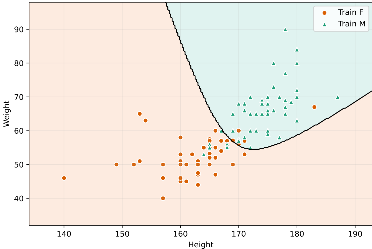
2D Gaussian Bayes Decision Boundary
