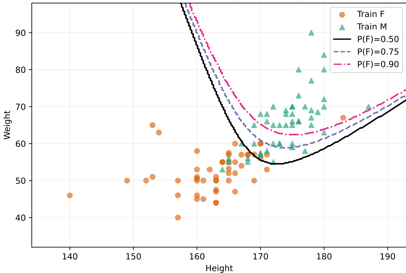
Effect of Priors on Bayes Boundary
