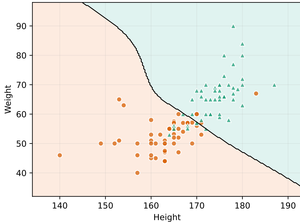
Parzen Bayes (h=5.0)
