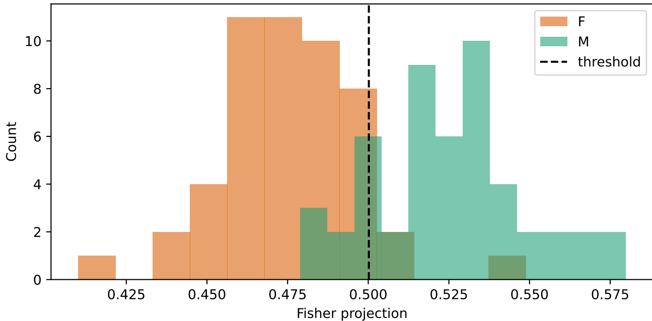
Training Samples on Fisher Projection
