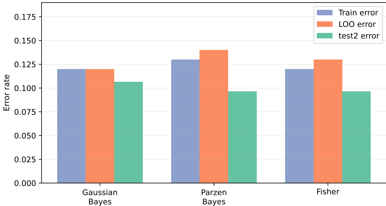
Training, Leave-one-out, and Test Error
