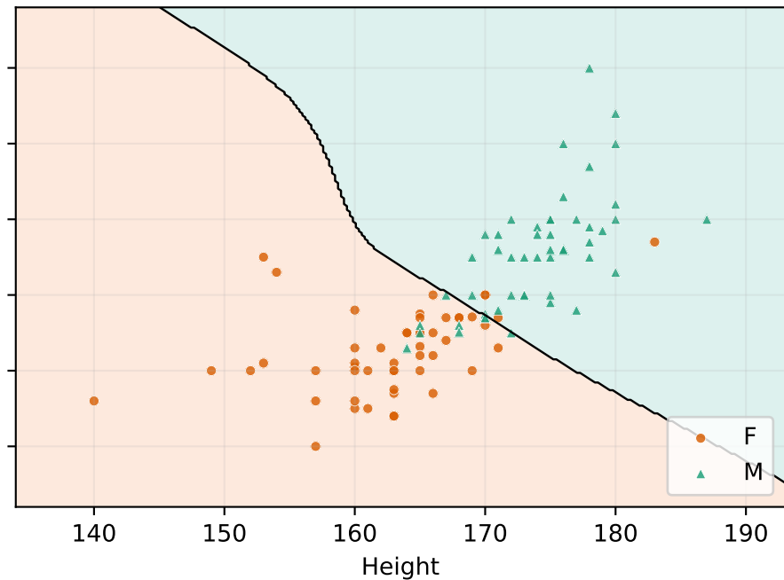
Parzen Bayes (h=5.0)
