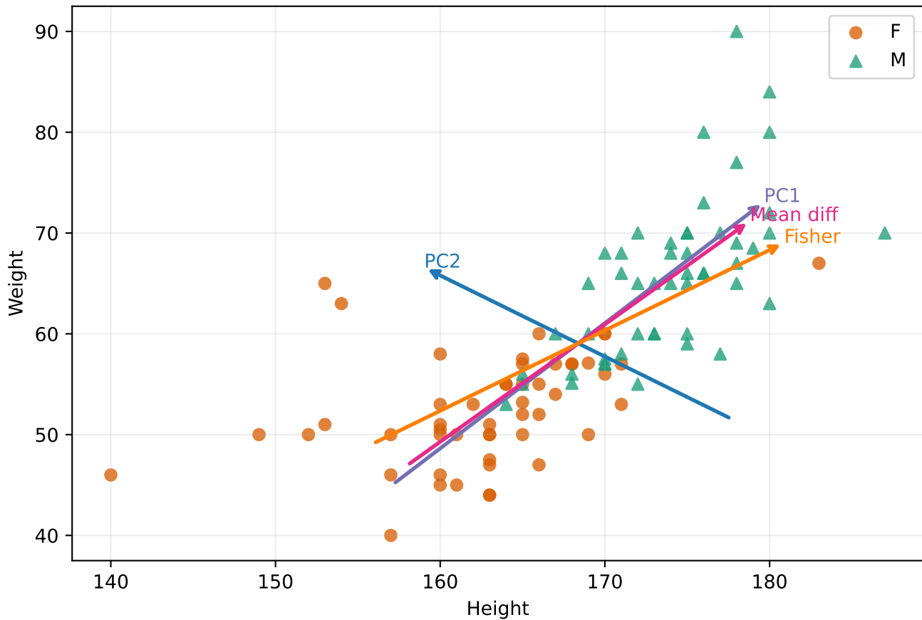
K-L Directions and Discriminant Directions
