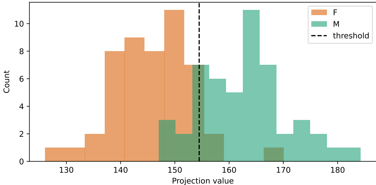
Projection on Class-Mean Difference Direction
