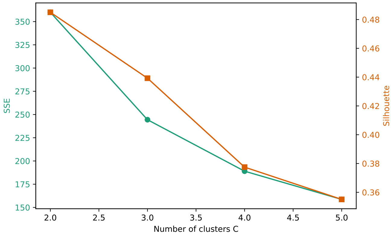
C-means Metrics on combined
