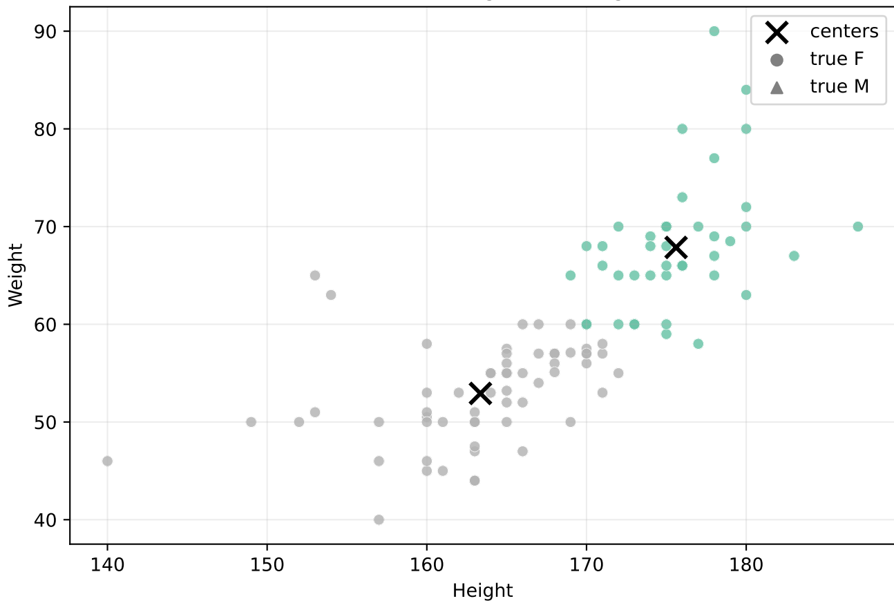
C-means Clustering on Training Data
